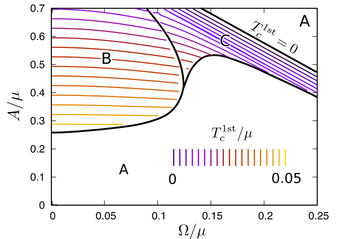
FIG. 4. Contour plot of the first order transition temperature T_c^{1st} . On the upper right boundary of the region C, the transition temperature reaches zero. In region A, there is no first order transition. For the second order transition temperature, see Fig. 2(d).
