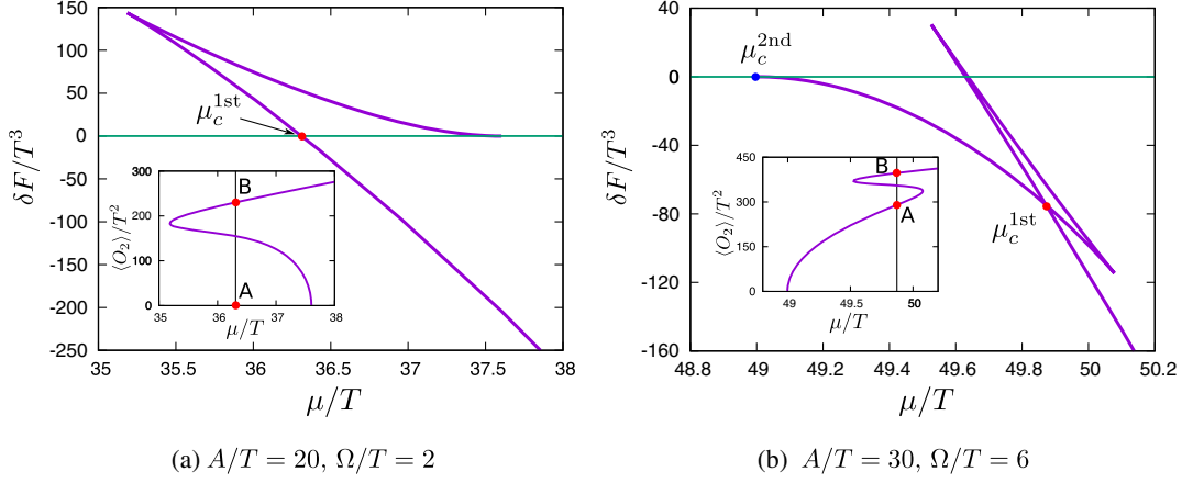
FIG. 7. Panels (a) and (b): Typical profiles of the free energy measured from the normal phase.
