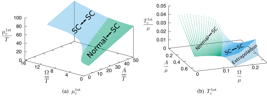
FIG. 8. Panel (a): The critical chemical potential \mu_c^{1st} for the first order phase transition. Panel (b): The critical temperature T_c^{1st} for the first order phase transition.
