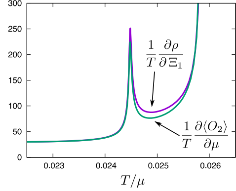
FIG. 9. Violation of the integrability conditions, evaluated when A/T = 20.94 , \Omega/T = 6.283 and \Xi_1 = 0 , which are the same parameters as in Fig. 3. The \Xi_1 -derivative is calculated around the trivial scalar source background. The divergence to the right is due to the superconducting phase transition and therefore is inessential.
