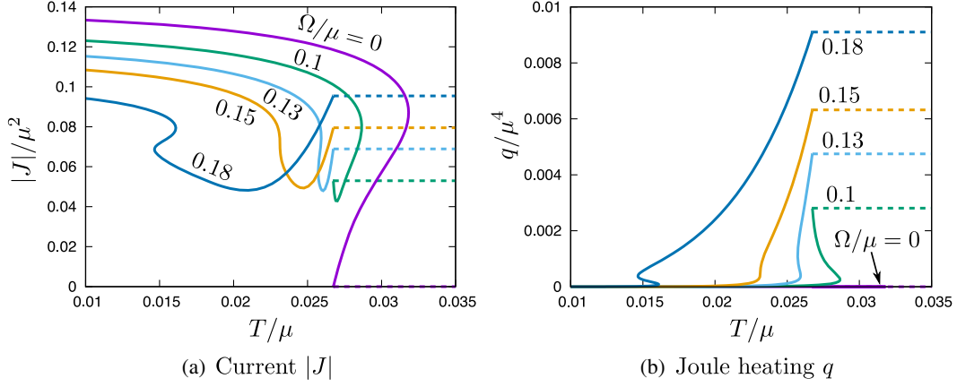
FIG. 5. Panel (a): Current J . Panel (b): Joule heating q . Both panels are plotted for A/\mu = 0.53 , \Omega/\mu = 0, 0.1, 0.13, 0.15, 0.18 . Dashed lines are normal phase values.
