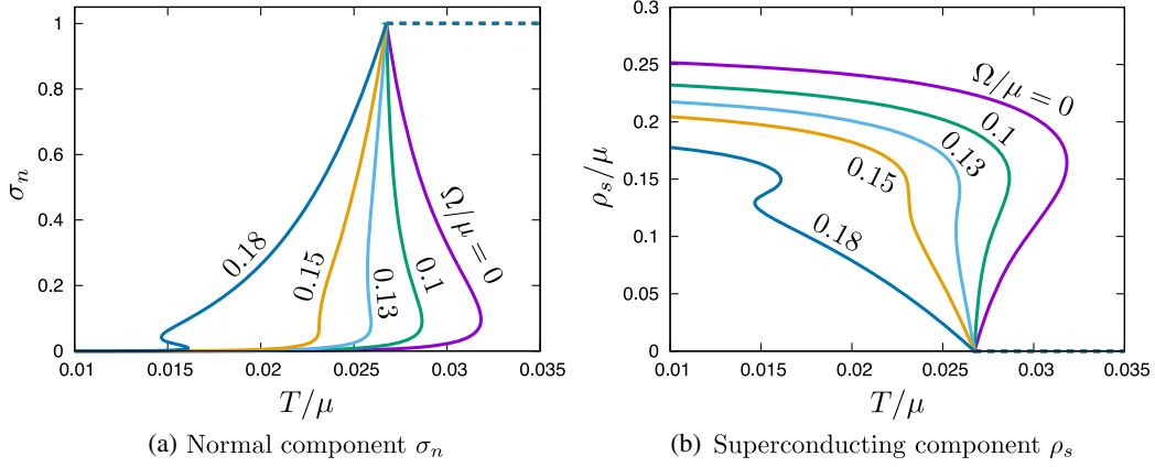
FIG. 6. Panel (a): The conductivity \sigma_n . Panel (b): The superfluid density \rho_s . Both panels are plotted for A/\mu = 0.53 and \Omega/\mu = 0, 0.1, 0.13, 0.15, 0.18 . Horizontal dashed lines in each panel indicate the normal phase values \sigma_n = 1 and \rho_s = 0 .
