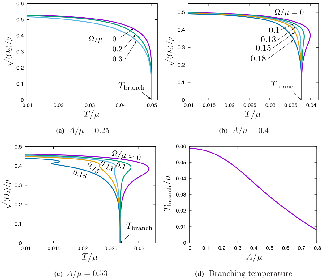
FIG. 2. Panels (a)–(c): Temperature dependence of the superconducting order parameter \sqrt{\langle O_2 \rangle} / \mu at A / \mu = 0.25, 0.4, 0.53 . Panel (d): The A / \mu -dependence of the branching temperature where \langle O_2 \rangle starts to become nonzero. This does not depend on \Omega for fixed A .
