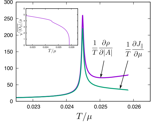
FIG. 3. Violation of the integrability condition \partial \rho / \partial |\vec{A}| = \partial J_{\parallel} / \partial \mu evaluated when A/T = 20.94 and \Omega/T = 6.283 . The chemical potential \mu is varied for a fixed temperature T . The inset shows the scalar condensate for these parameters.
