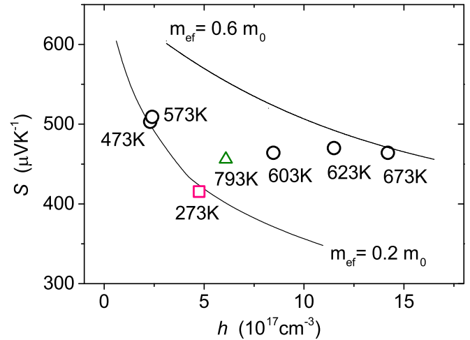
FIG. 13. The Seebeck coefficient S as a function of the Hall concentration of holes (Pisarenko plot) for various ATs (not shown are the samples annealed above the \alpha \rightarrow \beta transition temperature \approx 800 K). The solid lines are fits using a single parabolic model assuming scattering of FCs by acoustic phonons. The sample annealed at 793 K (green triangle) is on the verge of the \alpha \rightarrow \beta transition. The red square represents the standard (nonannealed) sample. The values were measured at T = 200 K.
