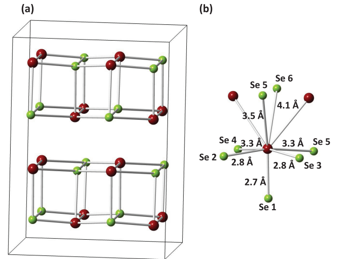
FIG. 1. (a) Structure of the SnSe Pnma phase; Sn and Se ions are indicated by red and green spheres, respectively. (b) Coordination of Sn ion. Interatomic distances between Sn and Se ions are denoted by labels.
