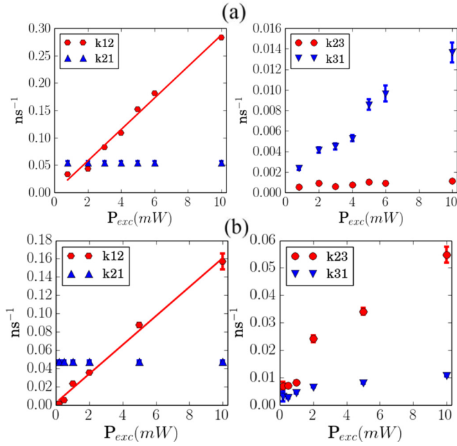
FIG. 6. (Color online) Evolution of k_{ij} parameters with power excitation when k_{21} is fixed for (a) the \text{NV}^0 and (b) the \text{NV}^- . Errors bars are shown where they exceed the symbol size. These error bars are estimated from those of the \gamma_1 , \gamma_2 , and \beta parameters; see Eqs. (14) to (16).
