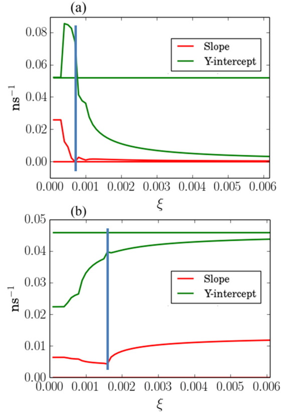
FIG. 7. (Color online) Evolution of the slope and the Y intercept of linear fit of k_{21}(P_{\text{exc}}) with the collection efficiency \xi for the \text{NV}^0 (a) and the \text{NV}^- (b). Straight lines are the values obtained previously with k_{21} fixed.
