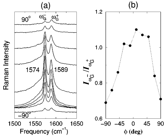
FIG. 4. (a) plots the G-band spectra for 10 different values of the angle \phi between the light polarization direction and the nanotube axis. (b) plots the integrated intensity ratio I_{\omega_G^-}/I_{\omega_G^+} as a function of \phi .
