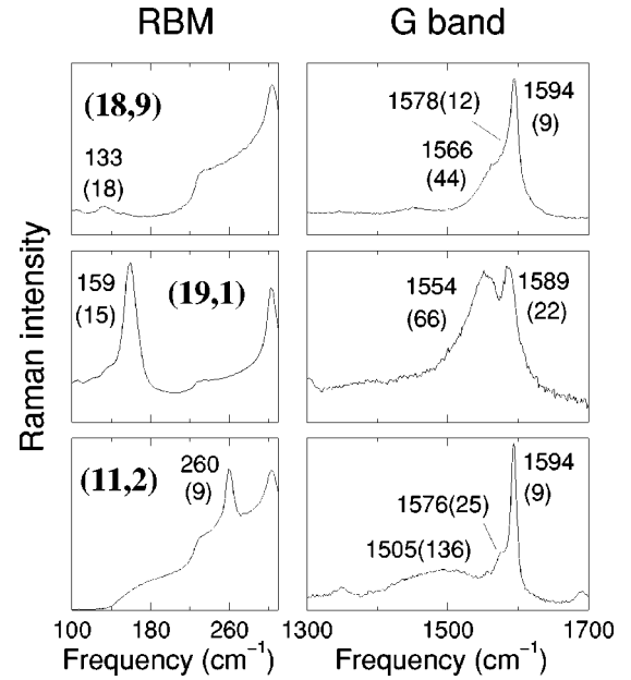
FIG. 2. The RBM and G-band Raman spectra for three isolated metallic SWNTs resonant with E_{\text{laser}} , that is, E_{\text{laser}} = 1.58 eV for the spectrum labeled (19,1), and E_{\text{laser}} = 2.41 eV for the other two spectra labeled (18,9) and (11,2). The spectra are taken at three different spots on the substrate. The frequencies (linewidths) of the peaks are displayed in \text{cm}^{-1} . The shoulder at 303 \text{ cm}^{-1} and the peak at 303 \text{ cm}^{-1} both come from the Si substrate.
