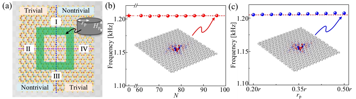
FIG. 5. (a) Within the shaded green (defect) zone, we introduce a number of rigid perturbation cylinders into the cavities where r_p and H_p are their radius and height. (b) Evolution of the corner states with the number of inserted cylinders N . (c) Same as (b), but here the radius of the perturbation cylinders r_p is increased. The red dashed line indicates the spectral location of the pristine corner state.
