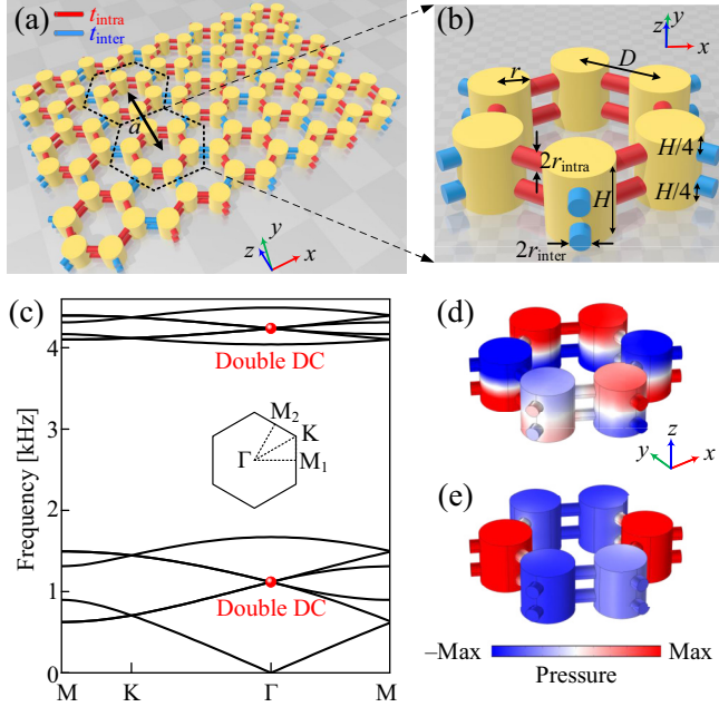
FIG. 1. (a) Schematic of the acoustic graphene-like honeycomb lattice, which is composed of identical cavity resonators (yellow) connected by variable coupling tubes (blue/red). (b) Enlarged view of the metamolecule. t_{\text{intra}} ( t_{\text{inter}} ) denote the intra- (inter-) metamolecular coupling strength that is controlled by the tube radius r_{\text{intra}} ( r_{\text{inter}} ). (c) Calculated band diagram of the lattice with r_{\text{intra}} = r_{\text{inter}} . Inset: First BZ. Pressure field of the acoustic modes corresponding to the (d) second and (e) first double Dirac cone. The color scale represents the total pressure field.
