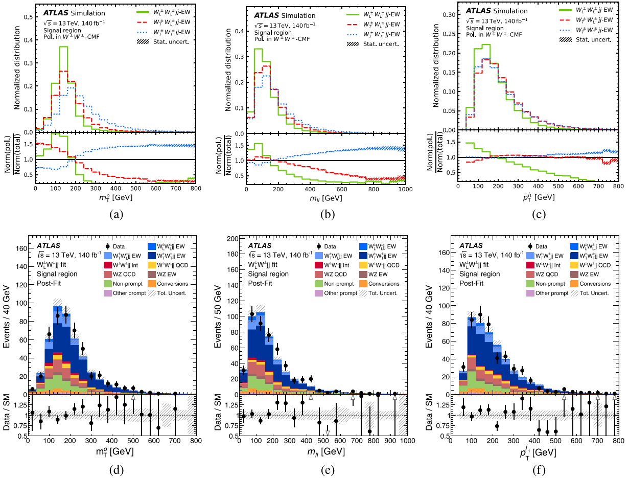
FIG. 4. Distributions in the SR for the [(a) and (d)] m_{\tau^0}^2 , [(b) and (e)] m_{\ell\ell} , and [(c) and (f)] p_T^{\text{J1}} . The ratios of the contributions of each process to the total contribution are shown in the bottom panels in (a)–(c). The predicted yields are shown with their best-fit normalization and shape in (d)–(f). The shaded area surrounding the expectation represents the total uncertainties in the predicted yields. The ratios of the observed yields to the total SM predictions are shown by the points in the bottom panels. The other prompt category combines ZZ , VVV , t\bar{t}V , and tZq background processes. The polarization vectors are defined in the W^+W^- center-of-mass reference frame.
