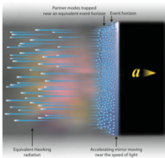
Accelerating mirror as an analog black hole
