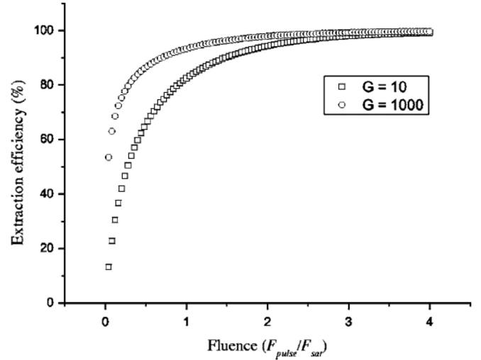
FIG. 2. Amplifier efficiency. This illustrates the importance for the input pulse fluence F_{\text{pulse}} to be a few times the saturation fluence F_{\text{sat}} to obtain a good extraction efficiency.
