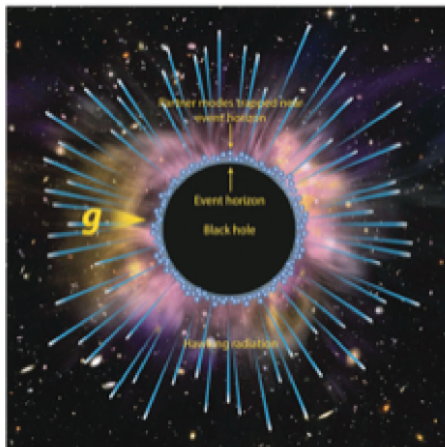
Black hole Hawking evaporation
