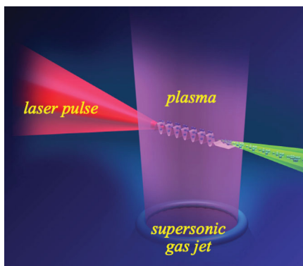
FIG. 13. The laser wakefield acceleration concept relies on the very large radiation pressure inducing a plasma wave. Electrons will be trapped in the wave and accelerated to energy of GeV/cm, 1000 times greater than conventional technology.
