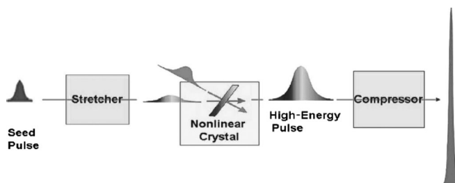
FIG. 9. OPCPA concept. In the OPCPA the pulse is amplified by optical parametric amplification instead of regular optical amplification. Note that for efficiency the pump pulse and the stretched pulse must have approximately the same duration and the same spatial extend.
