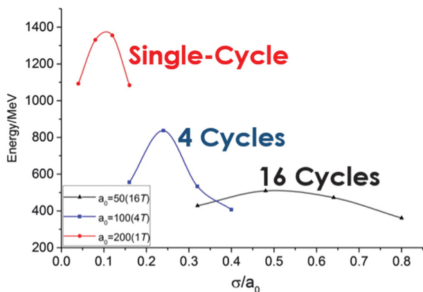
FIG. 15. In the single-cycle regime the acceleration efficiency of ions varies sharply. The fewer number of cycles translates into a larger laser vector potential and yields higher proton cutoff energy. The proton energy is increased by reducing the number of cycles from \tau = 16T (black curve) where T is the period to \tau = 4T (blue curve). In particular, with the single-cycle pulse (red curve), the cutoff energy of the ions is increased by a significant amount and becomes quickly relativistic.
