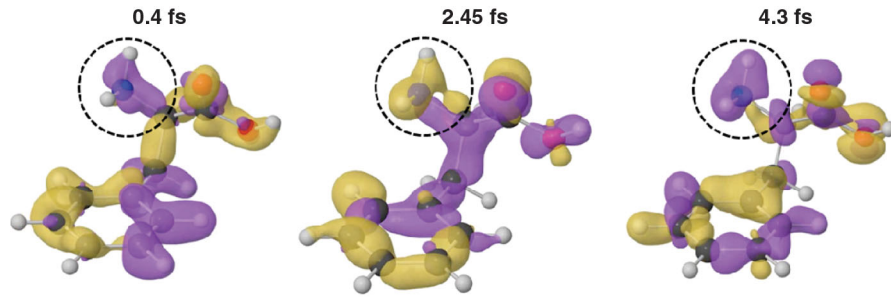
FIG. 16. Electron density around the amine group of phenylalanine changes sign in \sim 2 fs.
