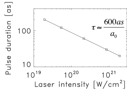
FIG. 12. Naumova, Nees, Hou et al. (2004) predicts a pulse duration scaling like T = 600 (attosecond)/ a_0 .
