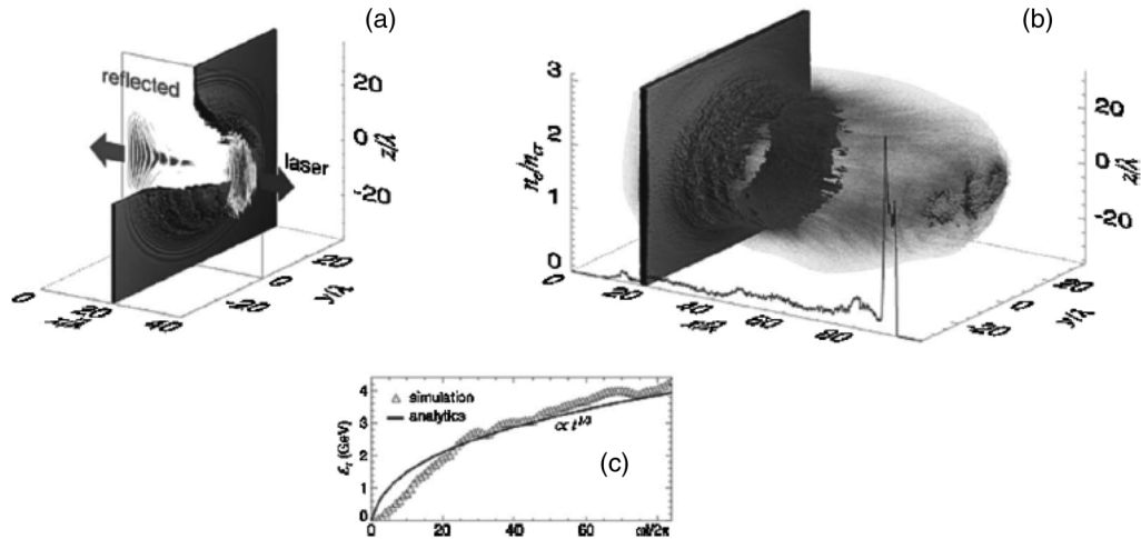
FIG. 14. In this regime for intensity in the 10^{23} W/cm 2 , the radiation pressure is dominant and scales with the laser-pulse energy.
