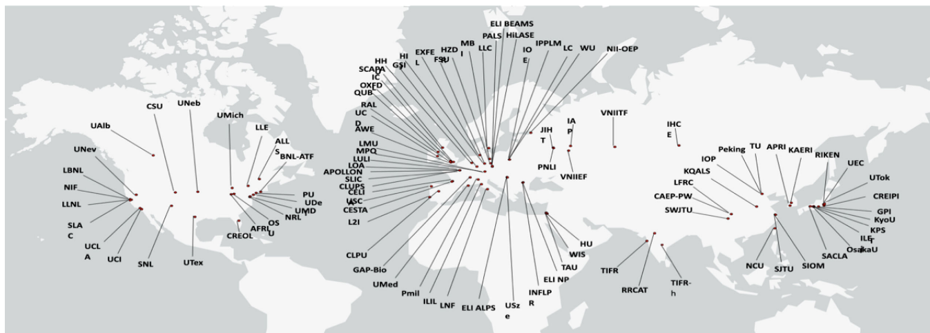
FIG. 7. World map of laser with peak power >100 TW.
