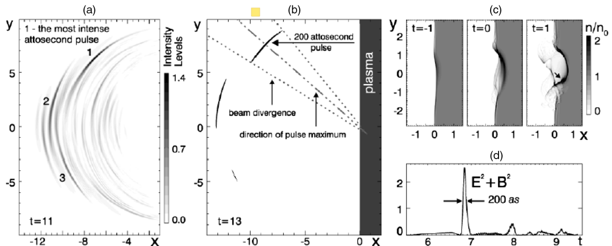
FIG. 11. The pulse is focused on \lambda^2 and creates a mirror with an indentation deforms due to (a). As it moves relativistically, it provides an isolated individual pulse (b), (c). (d) is the lineout through pulse one of (a).
