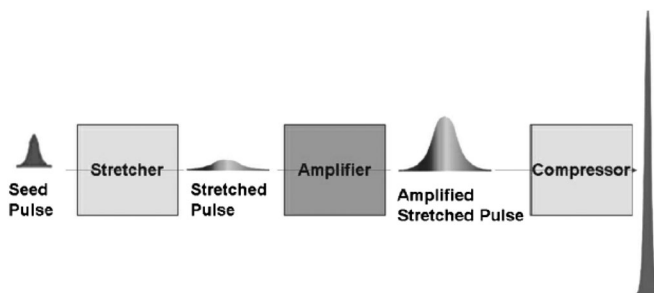
FIG. 4. Chirped pulse amplification concept. To minimize nonlinear effects the pulse is first stretched several thousand times lowering the intensity accordingly without changing the input fluence \text{J/cm}^2 . The pulse is next amplified by a factor of 10^6 – 10^{12} and is then recompressed by a factor of several thousand times closer to its initial value.
