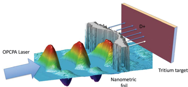
FIG. 19. Neutrons are generated by an OPCPA laser irradiation of a nanometric deuteron foil, deuteron acceleration and interaction with tritiated solid target. From Yan et al. , 2010.
