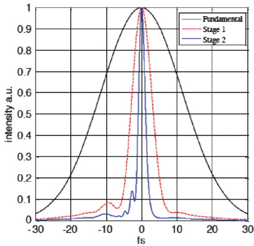
FIG. 10. This element uses a uniform thickness plastic element of around 0.5 mm. An incident flat top pulse will induce a uniform self-phase modulation across the element. After spectral broadening the pulse is compressed by two chirped mirrors to a near single-cycle pulse into a 2.1 fs after two compression stages.
