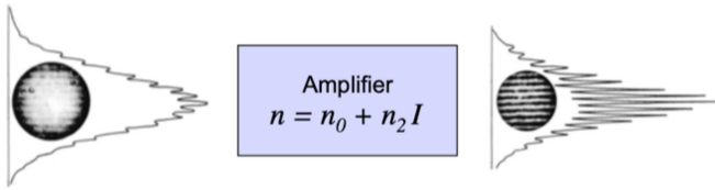
FIG. 3. The intensity dependence of the index of refraction will create spatial variation of the laser beam intensity, producing undesirable filaments and hot spot.
