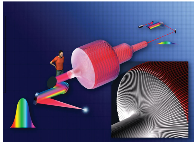
FIG. 6. The CAN system is a fiber-laser based system built out of thousands of fiber lasers coherently added to increase the average power and pulse energy linearly. The fiber laser offers excellent efficiency (>30%) thanks to laser-diode pumping and provides a much larger surface cooling area, therefore making operation at high peak power and high average power possible with good efficiency and pristine beam quality.
