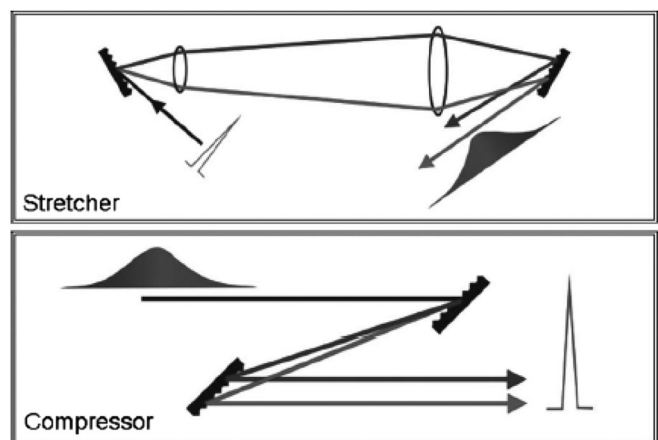
FIG. 5. Treacy and Martinez grating arrangements. The Martinez grating pair used as a stretcher and Treacy grating pair used as a compressor. It was discovered and demonstrated by Pessot et al. (1987) that these two grating arrangements are in fact matched over all orders. The pulse can be stretched and recompressed arbitrarily keeping the initial pulse unchanged. This grating arrangement is used in most CPA systems.
