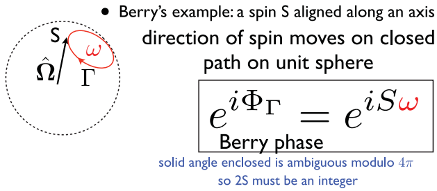
FIG. 3. Berry phase for the adiabatic evolution of the state of a quantum spin aligned along a moving axis. The Berry phase \Phi_\Gamma is the spin quantum number S times the solid angle subtended by the closed path \Gamma of the alignment axis \hat{\Omega} . After the axis returns to its initial orientation, the final quantum state is the initial state times the factor \exp i\Phi_\Gamma that depends geometrically on the path taken. Since the “solid angle subtended by the path” is ambiguous modulo 4\pi , 2S is topologically required to be an integer (which it is).
