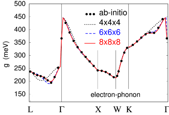
FIG. 6. Comparison between Wannier-interpolated electron-phonon matrix elements and explicit DFPT calculations for diamond. The interpolated matrix elements were calculated starting from a coarse 4^3 Brillouin-zone grid (dotted line, black), a 6^3 grid (dashed line, blue), and a 8^3 grid (solid line, red). The dots indicate explicit DFPT calculations. In this example |n\mathbf{k}\rangle is set to the valence band top at \Gamma ; |m\mathbf{k} + \mathbf{q}\rangle spans \Lambda_3 , \Delta_5 , and \Sigma_2 bands, and the phonon is set to the highest optical branch. From Giustino, Cohen, and Louie, 2007.
