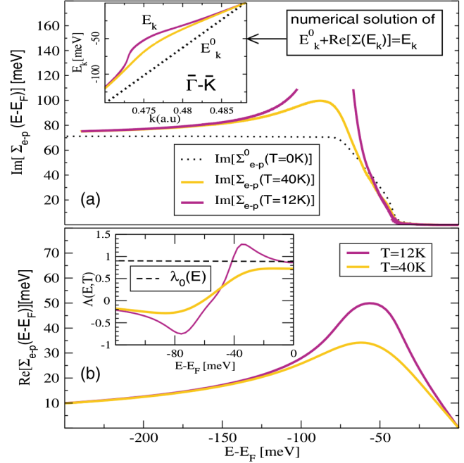
FIG. 11. Calculated Fan-Migdal self-energy of the surface state at the Be(0001) surface. (a) Imaginary part of the self-energy, obtained from Eq. (188). The dashed (black) line is the self-energy evaluated using the DFT-LDA bands; the solid lines (color, gray scale) correspond to the self-energy calculated by taking into account the renormalization of the DFT band structure by the electron-phonon interaction. (b) Real part of the self-energy, using the same color, gray scale code as in (a). The inset in (a) compares the renormalized band structure (color) with the ‘‘bare’’ DFT band (black dashed line). The inset of (b) shows the renormalization of the band velocity induced by the electron-phonon interaction. From Eiguren, de Gironcoli et al. , 2003.
