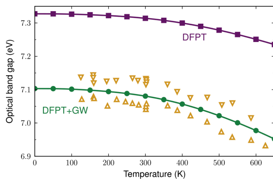
FIG. 13. Temperature dependence of the direct band gap of diamond calculated using the Allen-Heine theory. The upper curve shows the results obtained within DFPT at the LDA level. The lower curve was obtained via GW calculations in the frozen-phonon approach. Triangles are experimental data. The zero-point renormalization calculated by including GW quasiparticle corrections is 628 meV. From Antonius et al., 2014 .
