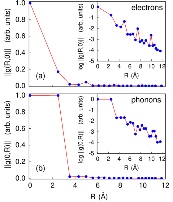
FIG. 5. Spatial decay of the electron-phonon matrix elements of diamond in the Wannier representation: (a) \max |g_{mn\kappa\alpha}(\mathbf{R}_p, 0)| vs |\mathbf{R}_p| , and (b) \max |g_{mn\kappa\alpha}(0, \mathbf{R}_{p'})| vs |\mathbf{R}_{p'}| . The maximum values are taken over all subscript indices, and the data are normalized to the largest value. The insets show the same quantities in logarithmic scale. The calculations were performed using the local density approximation to DFT. From Giustino, Cohen, and Louie, 2007.
