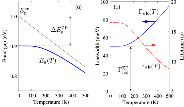
FIG. 3. Temperature-dependent band gap and lifetimes in an idealized semiconductor or insulator. (a) Temperature dependence of the band gap according to Eq. (168) (thick solid blue line). The straight thin black line is the asymptotic expansion at high temperature; this line intercepts the vertical axis at the band gap calculated with clamped nuclei E_g^{\text{cn}} . The difference between the latter value and the band gap at T = 0 including the EPI gives the zero-point renormalization \Delta E_g^{\text{ZP}} . (b) Temperature dependence of the electron linewidth (solid blue line) and lifetimes (dashed red line) using the same model as in (a). The zero-point broadening is \Gamma_{nk}^{\text{ZP}} . This simplified trend is valid only when the electron energy is at least one phonon energy away from a band extremum, so that both phonon emission and phonon absorption processes are allowed. The parameters of the model are E_g^{\text{cn}} = 1 eV, \Delta E_g^{\text{ZP}} = 100 meV, \hbar\omega_0 = 100 meV, and \Gamma_{nk}^{\text{ZP}} = 50 meV. These values are representative of common semiconductors.
