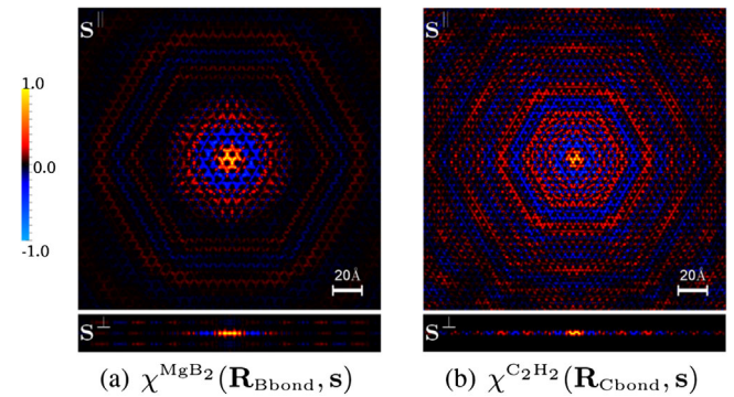
FIG. 18. Superconducting order parameter \chi(\mathbf{r}, \mathbf{r}') in real space, calculated for (a) \text{MgB}_2 and (b) hole-doped graphane. The plots show a top view (top) and a side view (bottom) of the hexagonal layers in each case. The variable \mathbf{s} = \mathbf{r} - \mathbf{r}' is the relative coordinate in the order parameter, while the center-of-mass coordinate is placed in the middle of a B-B bond or a C-C bond. From Linscheid, Sanna, Floris, and Gross, 2015.
