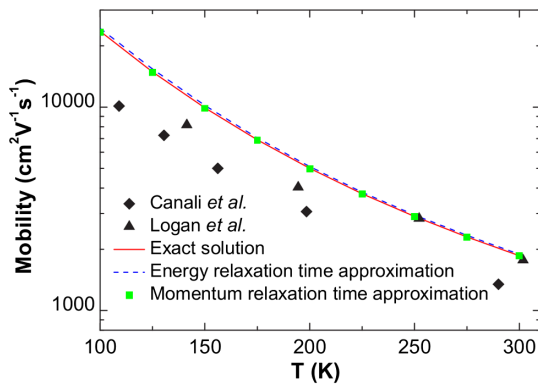
FIG. 16. Temperature-dependent mobility of n -type silicon. The solid line (red) indicates the mobility calculated using the linearized Boltzmann transport equation, Eq. (202), and the dashed line (blue) corresponds to the energy relaxation time approximation. The triangles and diamonds are experimental data points. From Li, 2015.
