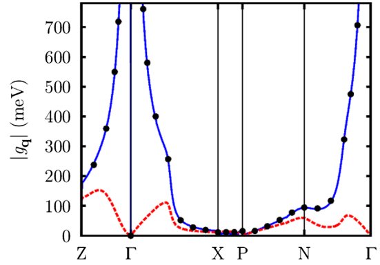
FIG. 7. Wannier interpolation of electron-phonon matrix elements for anatase \text{TiO}_2 . The initial state |n\mathbf{k}\rangle is set to the bottom of the conduction band at \Gamma , the final state |m\mathbf{k} + \mathbf{q}\rangle spans the bottom of the conduction band along high-symmetry lines, and the phonon is the highest LO mode. The dots correspond to explicit DFPT calculations. The red dashed line is the short-range component of the matrix elements g^{\text{S}} . The solid blue curve represents the matrix elements g^{\text{S}} + g^{\text{L}} , as obtained from the modified Wannier interpolation of Sec. VI.A.3. The interpolation was performed starting from a coarse 4 \times 4 \times 4 unshifted grid. From Verdi and Giustino, 2015.
