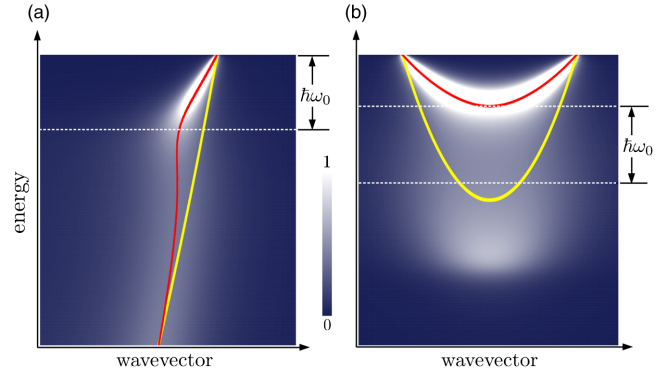
FIG. 4. Two-dimensional maps of the electron spectral function A(\mathbf{k}, \omega) for electrons coupled to a dispersionless phonon of frequency \omega_0 . The noninteracting bands are given by \varepsilon(\mathbf{k}) = -\varepsilon_F + \hbar^2 |\mathbf{k}|^2 / 2m^* , and the Fermi level coincides with the top of the energy window. The matrix element is |g|^2 = \hbar\omega_0 / N_F when the electron energies differ by less than the cutoff \varepsilon_{\text{max}} and zero otherwise ( N_F is the density of states at the Fermi level). (a) Spectral function for the case \varepsilon_F = 10\hbar\omega_0 (white on blue, black), noninteracting band structure (solid line, yellow, light gray), and fully interacting band structure within the Brillouin-Wigner perturbation theory (solid line, red, dark gray). (b) Spectral function for the case \varepsilon_F = 2\hbar\omega_0 . The model parameters are m^* = 0.1m_e , \hbar\omega_0 = 100 meV, \eta = 20 meV, and \varepsilon_c = 5 eV. For clarity the calculated spectral functions are cut off at the value 3 \text{ eV}^{-1} and normalized. The self-energy is shifted by a constant so as to have \Sigma^{\text{ep}}(0) = 0 . This correction guarantees the fulfillment of Luttinger’s theorem about the volume enclosed by the Fermi surface (Luttinger, 1960).
