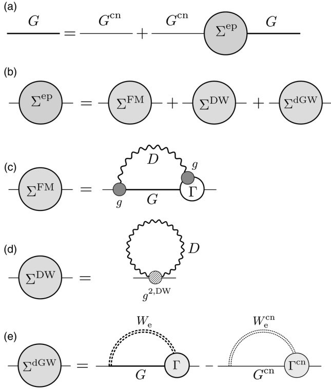
FIG. 2. Diagrammatic representation of the electron Green's function and electron-phonon self-energy. (a) Dyson equation for the electron Green's function, Eq. (151). The thick straight line represents the fully dressed electron propagator, the thin straight line is the propagator calculated at clamped nuclei, and the disk is the electron-phonon self-energy. (b) Decomposition of the electron-phonon self-energy into Fan-Migdal self-energy, Eq. (153), Debye-Waller contribution, Eq. (154), and the remainder given by Eq. (155). (c) Fan-Migdal electron-phonon self-energy expressed in terms of the dressed electron-phonon coupling function (dark gray disk as in Fig. 1), the fully interacting electron Green's functions (thick straight line), the fully interacting phonon propagator (thick wavy line), and the vertex \Gamma from Eq. (83). (d) Debye-Waller contribution resulting from the fully interacting phonon propagator (thick wavy line) and the matrix element in Eq. (40) (hatched disk). (e) Correction to Hedin's GW self-energy arising from the modification of the electronic structure induced by the electron-phonon interaction. W_e is the screened Coulomb interaction of Eq. (94) (bold dashed double line). W_e^{\text{cn}} is the screened Coulomb interaction evaluated at clamped nuclei (thin dashed double line). \Gamma^{\text{cn}} is the vertex of Eq. (83), but evaluated at clamped nuclei.
