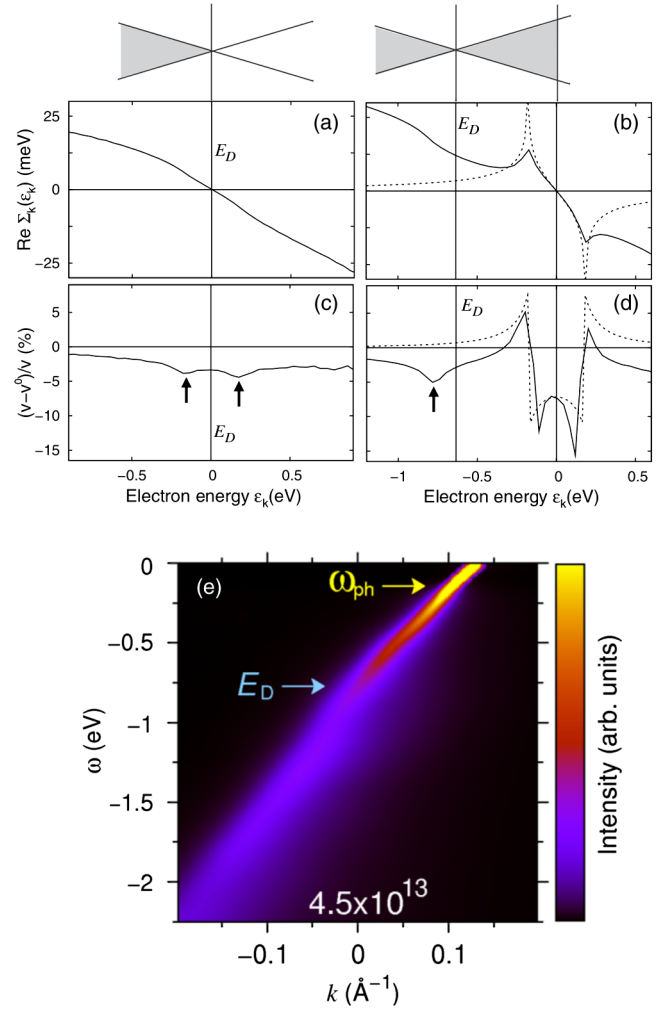
FIG. 12. (a), (b) Calculated real part of the Fan-Migdal self-energy in pristine and n -doped graphene, respectively (solid black lines). The doping level is 4 \times 10^{13} \text{ cm}^{-2} . The dashed lines correspond to a simplified analytical model where particle-hole symmetry is assumed. (c), (d) Electron band velocity renormalization resulting from the self-energies in (a) and (b). All calculations in (a)–(d) were performed using DFT-LDA. From Park et al. , 2007. (e) Calculated spectral function of n -doped graphene for one of the branches of the Dirac cone. \omega_{\text{ph}} indicates the characteristic phonon energy leading to the photoemission kink, and E_{\text{D}} denotes the energy of the Dirac point. The calculations include GW quasiparticle corrections. From Park et al. , 2009.
