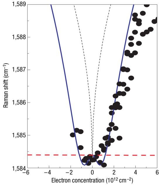
FIG. 8. Frequency of the Raman G band of graphene vs carrier concentration. The black filled disks are from Raman measurements of gated graphene on a silicon substrate at 295 K. The thick horizontal dashed line (red) shows the variation of the E_{2g} mode frequency with doping, within the adiabatic approximation. The solid blue line shows the variation of the frequency calculated by including nonadiabatic frequency renormalization. From Pisana et al. , 2007 .
