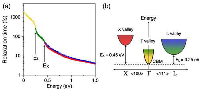
FIG. 15. Electron relaxation times in GaAs resulting from electron-phonon scattering. (a) Calculated relaxation times as a function of electron energy with respect to the conduction band bottom. The color code (gray shades) of the data points identifies the valley where each electronic state belongs. (b) Schematic representation of the conduction band valleys in GaAs. From Bernardi et al. , 2015 .
