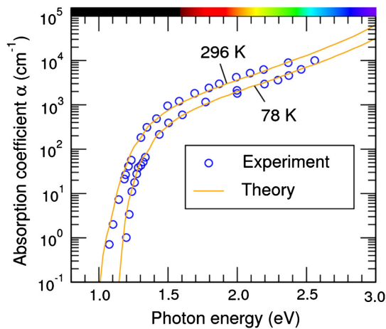
FIG. 14. Phonon-assisted optical absorption in silicon: comparison between first-principles calculations (solid lines, orange) and experiment (circles, blue). The calculations were performed using the theory of Hall, Bardeen, and Blatt (1954), as given by Eq. (200). Spectra calculated at different temperatures were shifted horizontally so as to match the experimental onsets. From Noffsinger et al. , 2012.
