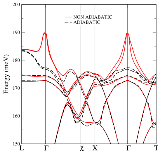
FIG. 10. Phonon dispersion relations of \text{CaC}_6 calculated using Wannier interpolation. The dashed lines (black) and the solid lines (red) represent the standard adiabatic calculation and the nonadiabatic phonon dispersions, respectively. From Calandra, Profeta, and Mauri, 2010.
