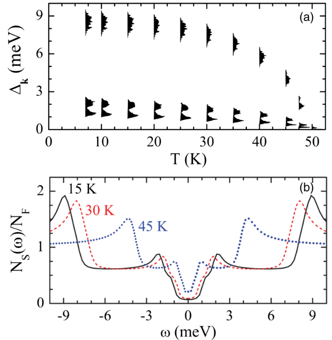
FIG. 17. (a) Energy distribution of the superconducting gap function of MgB 2 as a function of temperature, calculated using the anisotropic Migdal-Eliashberg theory. The gap vanishes at the critical temperature (in this calculation T_c = 50 K). Two distinct superconducting gaps can be seen at each temperature. (b) Density of electronic states in the superconducting state of MgB 2 at various temperatures calculated within the Migdal-Eliashberg theory. From Margine and Giustino, 2013.
