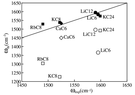
FIG. 9. Comparison between measured ( \omega_{\text{exp}} ) and calculated ( \omega_{\text{th}} ) vibrational frequencies of the E_{2g} mode of graphite intercalation compounds. Open symbols are adiabatic DFPT calculations, and filled symbols are calculations including the nonadiabatic corrections. The line corresponds to \omega_{\text{th}} = \omega_{\text{exp}} . From Saitta et al. , 2008 .
