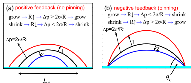
FIG. 35 (color online). Stabilization mechanism of evaporating surface nanodroplets in an oversaturated gas atmosphere through pinning: In (a) the droplet is not pinned, leading to a diverging Laplace pressure and thus evaporation of the droplet for any oversaturation. The equilibrium situation with footprint diameter L_e [Eq. (39), black curve] is unstable. In (b) the droplet is pinned. The equilibrium situation with contact angle \theta_e [Eq. (30), black curve] is stable. Adapted from Liu and Zhang, 2013a.
