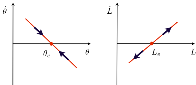
FIG. 34 (color online). (Left) Sketch of the stable equilibrium \theta_e for pinned surface nanobubbles in the \dot{\theta} vs \theta phase space. A sketch of the volume phase space \dot{V} vs V or of the bubble height phase space \dot{H} vs H looks the same. (Right) Sketch of the unstable equilibrium L_e for unpinned surface nanobubbles with constant contact angle in the \dot{L} vs L phase space. A sketch of the volume phase space \dot{V} vs V looks the same. Also for bulk bubbles, the sketch looks the same, with the lateral extension L then meaning the bubble diameter or being replaced by the radius R or the volume V of the bulk bubble. From Lohse and Zhang, 2015.
