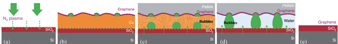
FIG. 38 (color online). Illustration of the transferring process of graphene from copper to SiO 2 facilitated by nanobubbles. (a) The supporting substrate SiO 2 /Si was pretreated by nitrogen plasma to convert the top layer of SiO 2 /Si to silicon oxynitride phases. (b) The substrate was coated with a copper film and then a graphene film was prepared by chemical vapor deposition onto the copper layer. Some bubbles were trapped during the graphene growth process. (c) After a layer of PMMA was coated on graphene for protection, the copper layer was dissolved in an etching solution. A silicon oxynitride phase readily decomposes, serving an additional source for nanobubbles. (d) Nanobubbles form under the graphene film. The capillary forces created by nanobubbles held the soft PMMA film and the graphene down to the hard supporting substrate. Throughout the etching process the PMMA-graphene film adhered firmly to the underlying substrate. (e) Once the solution and PMMA were washed off, the face-to-face transfer was completed. From Gao et al. , 2014.
