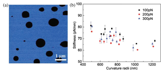
FIG. 23 (color online). Stiffness of nanobubbles measured by AFM in the mode of peak force QNM. (a) Stiffness image. The shaded area is the hard HOPG substrate, and the black circular regions are soft nanobubbles. (b) The nanobubble stiffness vs their curvature radii. The nanobubbles behave like a Hook spring. Bigger nanobubbles are always “softer” than smaller ones. From Zhao et al. , 2013.
