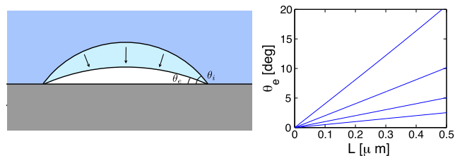
FIG. 32 (color online). (Left) Sketch of the shrinking process of a pinned surface nanobubble with footprint diameter L and initial contact angle \theta_i > \theta_e toward the equilibrium contact angle \theta_e . (Right) Equilibrium contact angle \theta_e of a nitrogen bubble in water as a function of the lateral footprint size L for four different oversaturations \zeta = 0.25, 0.5, 1.0, 2.0 , bottom to top. From Lohse and Zhang, 2015.
