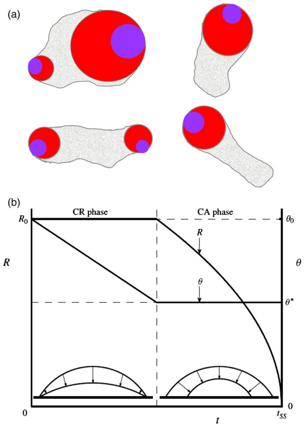
FIG. 36 (color online). (a) Top-view sketch of patches of chemical heterogeneities (light shaded) on the surface. They are more hydrophobic and surface nanobubbles or nanodroplets (larger shaded circles) adhere to them. If exposed to a (partly) degassed or undersaturated water environment ( c_\infty < c_s or \zeta < 0 ), the nanobubbles (or nanodroplets) shrink, first in the constant footprint mode (CR mode) due to the pinning, and then jump toward a smaller footprint (CA mode), as drawn by the smaller shaded nanobubbles and nanodroplets. (b) Scheme of a shrinking droplet in the stick-slip mode. The drop transitions from the constant (footprint) radius mode (CR) to the constant contact angle mode (CA). From Stauber et al. , 2014. More realistically, the jump in the CA will be only on one side, due to in general different pinning strengths on the two sides, leading to a shift in the center of mass, as shown in (a).
