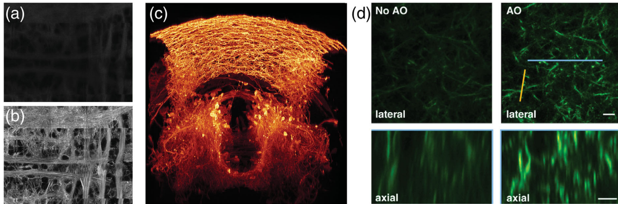
FIG. 22 (color). Adaptive optics enables deep imaging at high resolution. (a) Two-photon image of membrane-labeled neurons in the spinal cord of a live zebrafish embryo, 72 hours post fertilization. (b) Same region after adaptive optical correction using direct wavefront sensing (Wang et al. , 2014), demonstrating recovery of signal and spatial resolution. (c) Adaptive optical correction of a sparse subset of neurons over a large portion of the zebrafish brain. (d) In vivo two-photon lateral and axial views of neural processes deep in the mouse cortex, before (left) and after (right) adaptive optical correction using indirect wave front sensing (Ji, Sato, and Betzig, 2012).
