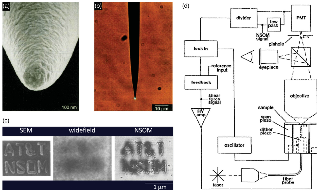
FIG. 5 (color). Making NSOM a real tool. (a) Electron micrograph and (b) optical micrograph of an adiabatically tapered, aluminum coated single mode optical fiber used as a near-field probe (Betzig and Trautman, 1992). (c) Resolution comparisons with the probe. Left to right: electron, conventional optical, and near-field optical micrographs (Betzig et al. , 1991). (d) Schematic diagram of shear force feedback for regulating, at the nm scale, the distance from the aperture at the end of the probe to the specimen (Betzig, Finn, and Weiner, 1992).
