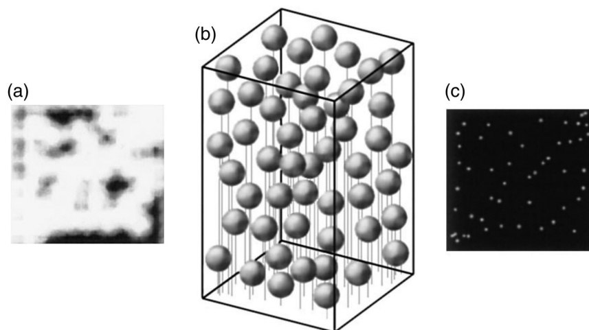
FIG. 11. The concept of super-resolution localization microscopy. (a) A field of close-packed molecules unresolved, because their diffraction-limited images overlap. (b) The same molecules, after their mutual isolation in a higher dimensional space. (c) Super-resolution map of molecular positions after localization of each isolated molecule. From Betzig, 1995 .
