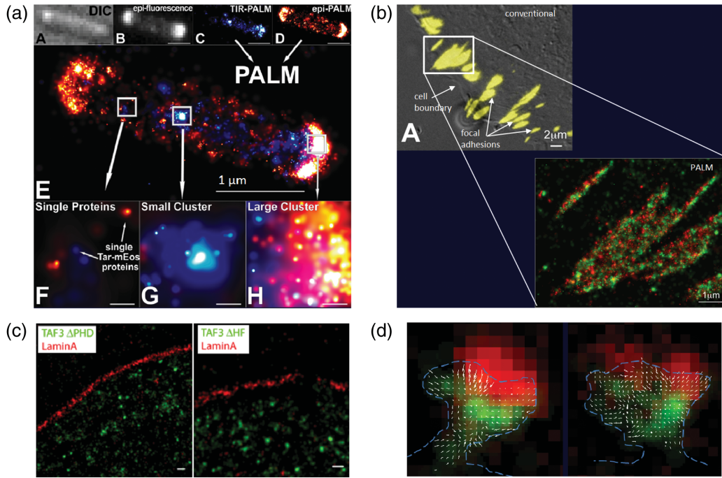
FIG. 17 (color). Applications of PALM. (a) Chemotaxis receptor clusters in E. coli (Greenfield et al. , 2009). (b) Two-color diffraction-limited and PALM views of the spatial relationship of vinculin and paxillin in focal adhesions (Shroff et al. , 2007). (c) Spatial relationship of core promoters of transcription (green) relative to the nuclear membrane (red) at different stages of myogenesis (Yao et al. , 2011). (d) Tracks of actin polymerization in dendritic spines of live cultured neurons (Frost et al. , 2010).
