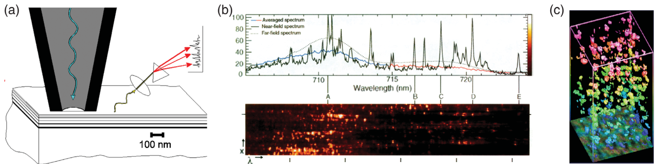
FIG. 10 (color). Near-field cryogenic spectroscopy of quantum wells. (a) Experimental schematic, showing a near-field probe (left) exciting a multiple quantum well structure (bottom), with the resulting emission measured at a spectrometer (right). (b) Comparative near-field and far-field spectra at a single point (top), and spectral changes with position (bottom). (c) Images of emission from single exciton recombination sites isolated from one another in a 3D space of position x , y and wavelength \lambda . From Hess et al. , 1994 .
