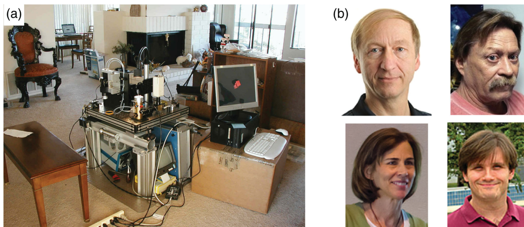
FIG. 14 (color). The development of PALM. (a) La Jolla Labs, also known as Harald's living room. (b) The PALM team. Clockwise from upper left: Harald Hess, Mike Davidson, George Patterson, and Jennifer Lippincott-Schwartz.
