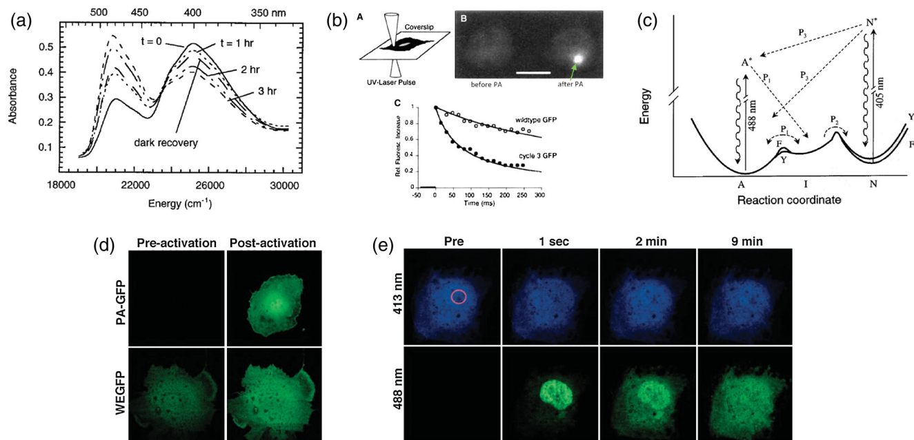
FIG. 13 (color). The development of photoactivatable GFP (PA-GFP). (a) UV-visible double absorption peaks of wild type GFP (Chattoraj et al. , 1996). (b) Pulse-chase experiment to trace the fate of wild type GFP locally photoactivated in one region of a cell (Yokoe and Meyer, 1996). (c) Energy state diagram from single-molecule photoactivation of GFP (Dickson et al. , 1997). (d) Improved on/off contrast ratio of PA-GFP (Patterson and Lippincott-Schwartz, 2002). (e) Pulse-chase experiment of the relative rates of nuclear and cytosolic diffusion of PA-GFP (Patterson and Lippincott-Schwartz, 2002).
