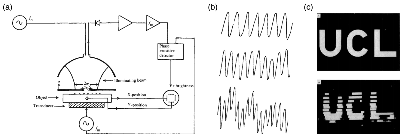
FIG. 2. Breaking the diffraction barrier in the near field. (a) Microwave resonator with subwavelength aperture as used by Ash and Nicholls (1972). (b) Resolved gratings having periods of 1/30 , 1/40 , and 1/60 (top to bottom) of the 3 cm microwave wavelength. (c) Images of letters having linewidths of 1/15 of the wavelength.
