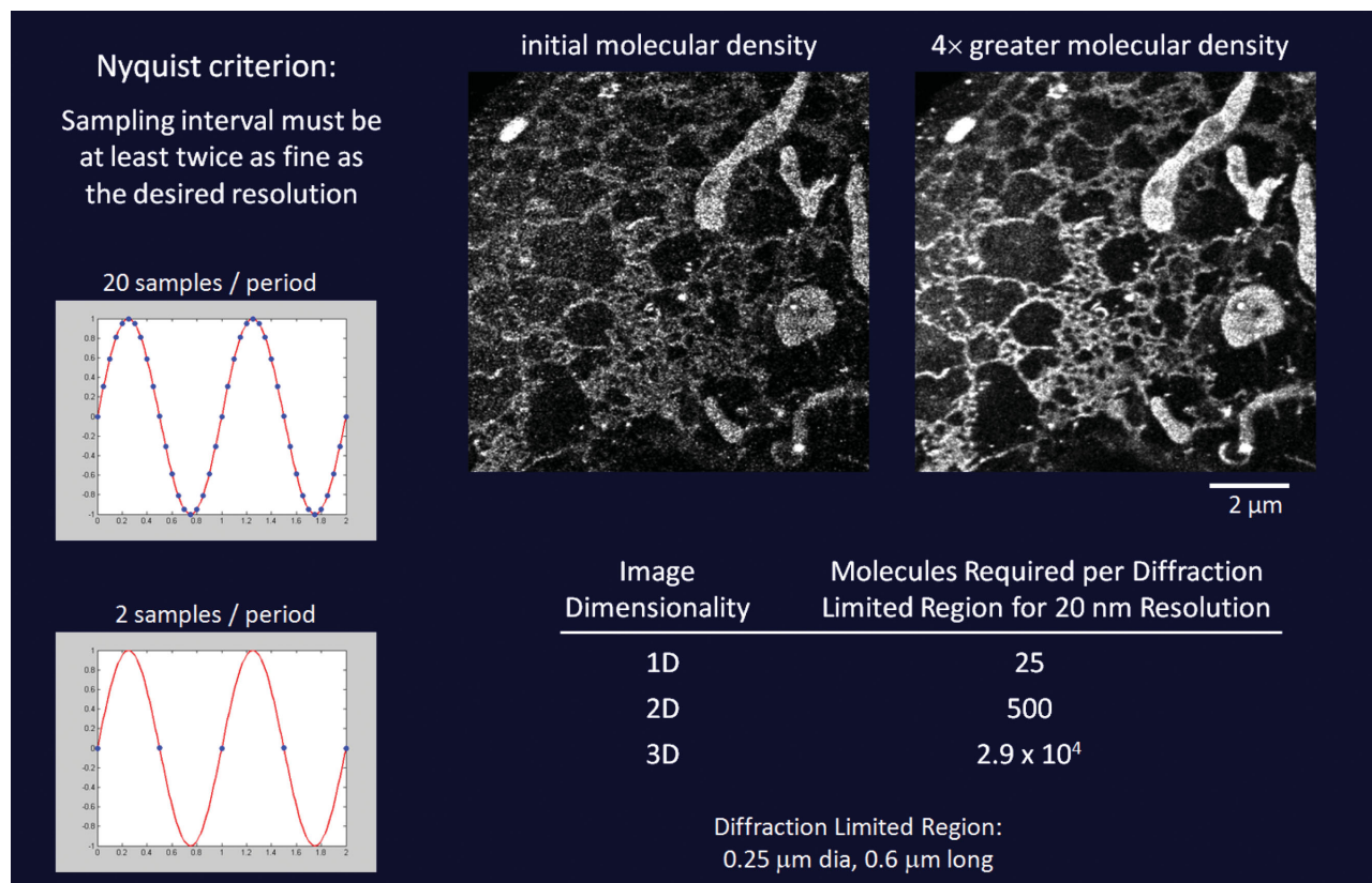
FIG. 12 (color). The Nyquist criterion and the labeling density problem. With many localized molecules per period, any spatial frequency is easily detectable (center left), but when the number drops to 2 per period or less, the frequency might be missed. As a result, resolution in localization microscopy is limited more by density of single-molecule labels than by the precision of their localization (top right). The minimum number of localizations required per diffraction-limited region increasing rapidly with dimensionality (lower right).
