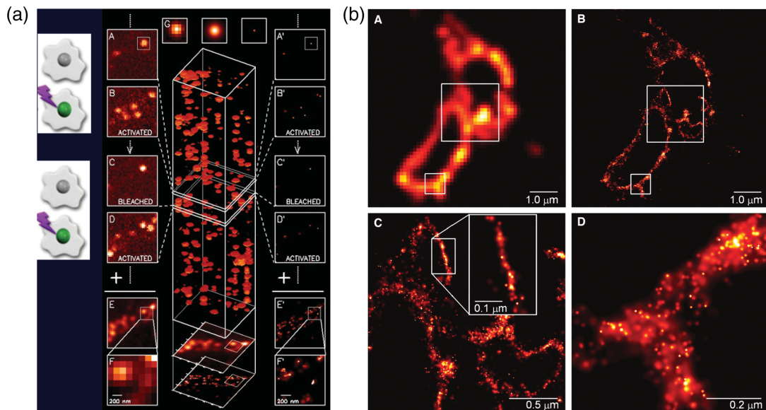
FIG. 15 (color). Photoactivated localization microscopy (PALM). (a) Repeated rounds of weak photoactivation with violet light activates different subsets of molecules in a specimen. Summing their diffraction-limited spots produces a diffraction-limited image (left column), but summing the measured centers of all such spots produces the super-resolution PALM image (right column). (b) Diffraction-limited (upper left) and super-resolution PALM images in different regions, showing the distribution of transmembrane protein CD-63 in a 70 nm section cut through lysosomes in a COS-7 cell. From Betzig et al. , 2006 .
