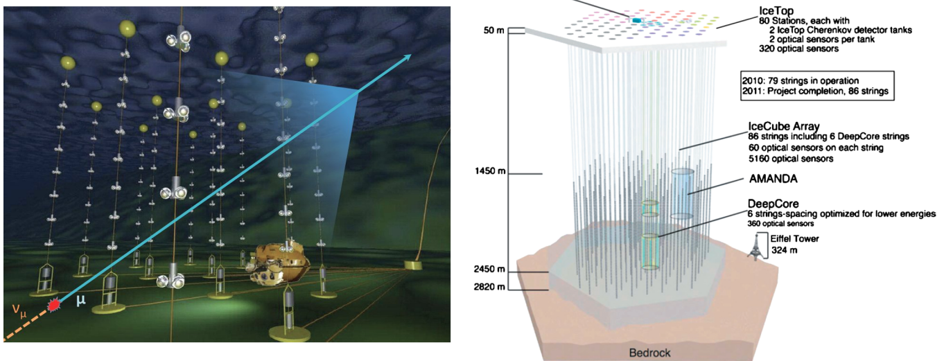
FIG. 6 (color online). Left: Schematic view of the ANTARES detector, with an illustration of its detection principle: an upgoing \nu_\mu interacting with matter in the seabed will produce a muon that can cross the detector, emitting a cone of Cherenkov light that will be detected by the array of photosensors. ANTARES consists of 12 instrumented lines anchored to the seabed at a depth of 2475 m, about 40 km off the coast of Toulon (France). The lines are 450 m long and kept up by a buoy; each of them supports 25 detection storeys separated by 14.5 m and supporting triplets of optical modules looking 45^\circ downward. The interline separation is about 70 m. Adapted from http://antares.in2p3.fr . Right: Schematic view of the IceCube detector at the South Pole. The strings are deployed from the surface and instrumented between 1450 and 2450 m; every string supports 60 optical modules enclosing one downward-looking PMT each. The interline separation is about 125 m. The sketch also shows the position of the prototype detector AMANDA, of the low-energy infill DeepCore, and of the surface array IceTop. From http://icecube.wisc.edu .
