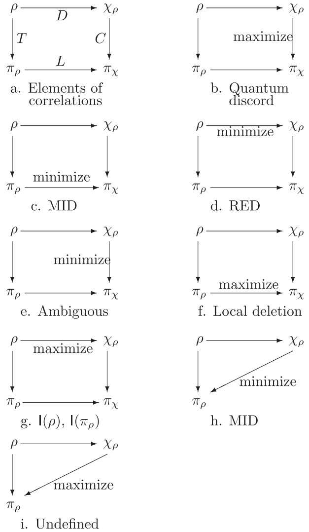
FIG. 4. Diagrammatic unification. Various possibilities to construct measures of quantum correlations. (a) The fundamental elements needed in defining a measure of correlations, namely, the discord D , classical correlations C , total correlations T , and a fourth quantity L . In each case, the distance is measured using relative entropy, and the closest state is given by maximizing or minimizing one distance as seen in (b)–(i). The relationship between \rho and \pi_\rho is fixed, so the total correlations are in all cases given by the mutual information. (b) Quantum discord is obtained when classical correlations are maximized. (c) Measurement-induced disturbance (MID) is obtained when the distance between the marginal states is minimized. (d) Relative entropy of discord (RED) is obtained by minimizing the distance between \rho and its classical state \chi_\rho . (e) This measure is not well defined. (f) Deleting local information by local measurements, however, some correlations may survive. (g) Information as defined in Sec. II.B. (h) Measurement-induced disturbance (MID). (i) This can be well defined, but has not been used previously. Adapted from Modi and Vedral, 2011.
