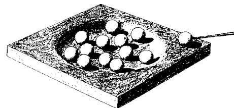
FIG. 4. Wooden toy model simulating Bohr's compound nucleus. Ref.: Nature 137 , 351 (1936).
