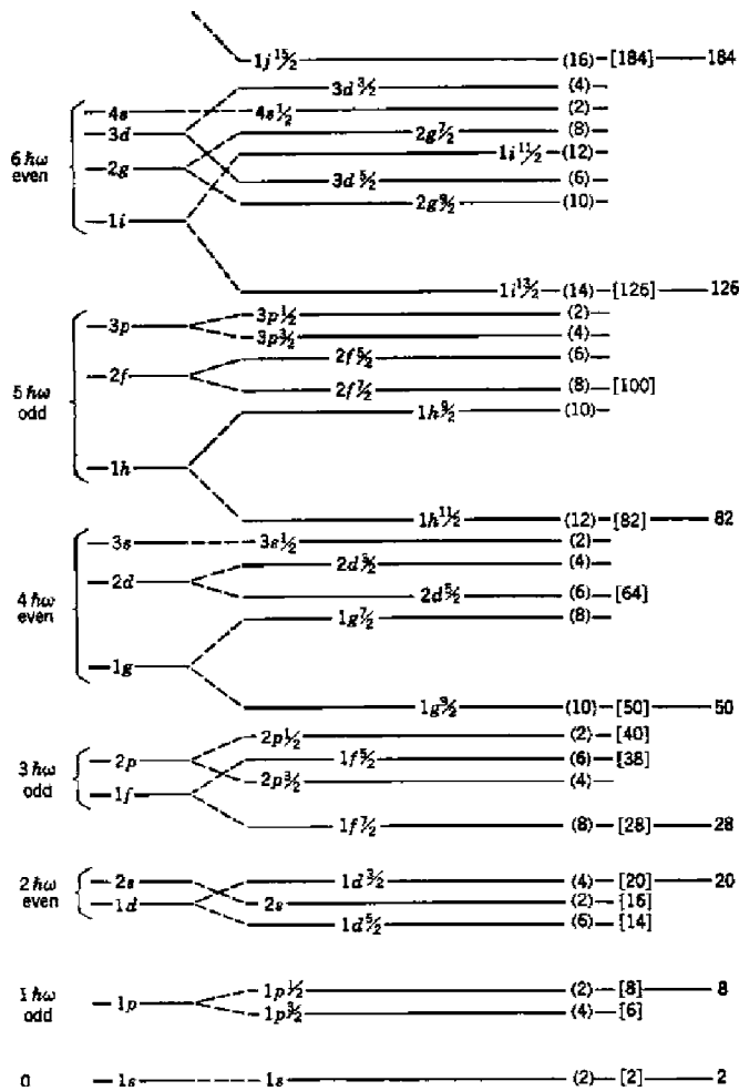
FIG. 10. Level sequence in the nuclear shell model. The orbitals are labeled by their spectroscopic notation, and the number of available single-particle states is shown. From Mayer and Jensen, 1955.
