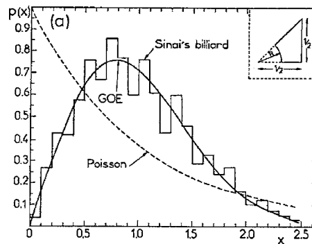
FIG. 6. The NNS distribution for the Sinai billiard (histogram) and the GOE prediction (solid line). From Bohigas et al. , 1986.
