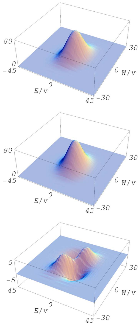
FIG. 19. (Color online) Same as Fig. 18 except for the correlations between the level densities for states with spin 0 and isospin 0 in ^{20}\text{Ne} and in ^{24}\text{Mg} . Left panel: Mean value of the product of the two level densities. Middle panel: Product of the mean level densities. Right panel: The correlator of Eq. (17) (from 400 realizations of the ensemble). From Papenbrock and Weidenmüller, 2006.
