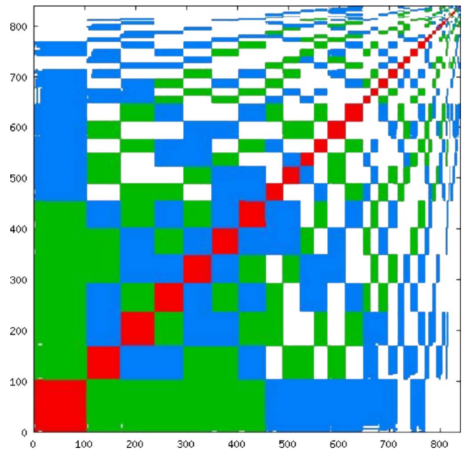
FIG. 13. (Color online) The block structure of the matrices C_{\mu\nu}(J, \alpha) for m=12 nucleons in the sd shell coupled to total spin J=0 and total isospin T=0 . Black (color online: red), no change of partition. Light gray (color online: green), change of partition by moving one nucleon. Dark gray (color online: blue), change of partition by moving two nucleons. White: there is no two-body matrix element that connects the states in question. From Papenbrock and Weidenmüller, 2005 .
