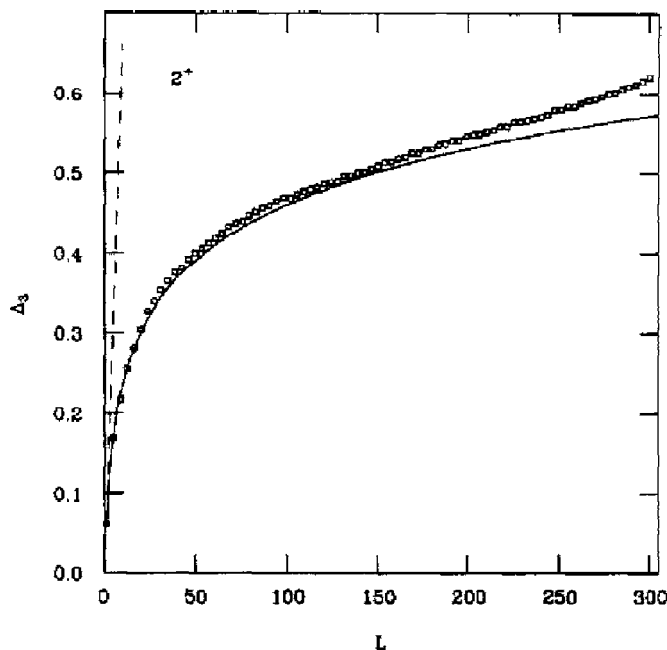
FIG. 12. The \Delta_3 statistic for the J=2 , T=0 states of 12 nucleons in the sd shell (data points) compared to the GOE (solid line). From Zelevinsky et al. , 1996.
