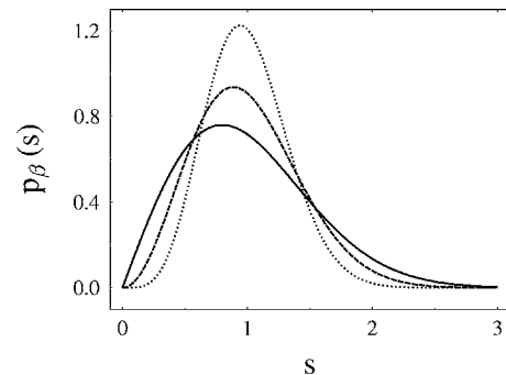
FIG. 5. The nearest-neighbor spacing distribution P_\beta(s) vs s , the actual spacing in units of the mean level spacing, for the three canonical ensembles with \beta=1, 2 , and 4 (solid, dashed, and dotted lines, respectively). \beta=2 corresponds to the GOE. From Guhr et al. , 1998.
