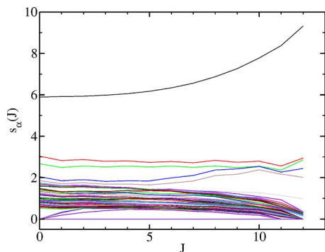
FIG. 14. (Color online) Roots s_\alpha(J) of the eigenvalues s_\alpha^2(J) defined in Eq. (8) vs total spin J for the T=0 states in ^{24}\text{Mg} . From Papenbrock and Weidenmüller, 2006.
