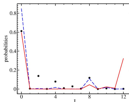
FIG. 17. (Color online) Same as Fig. 16 for the T=0 states in ^{24}\text{Mg} . From Papenbrock and Weidenmüller, 2006.
