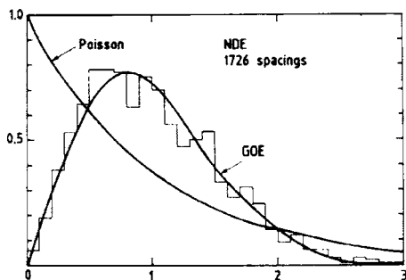
FIG. 8. The NNS distribution for the nuclear data ensemble (histogram) and the GOE prediction (solid line). From Haq et al. , 1983.
