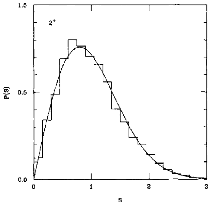
FIG. 11. The NNS spacing distribution for the J=2 , T=0 states of 12 nucleons in the sd shell (histogram) compared to the GOE (line). From Zelevinsky et al. , 1996.
