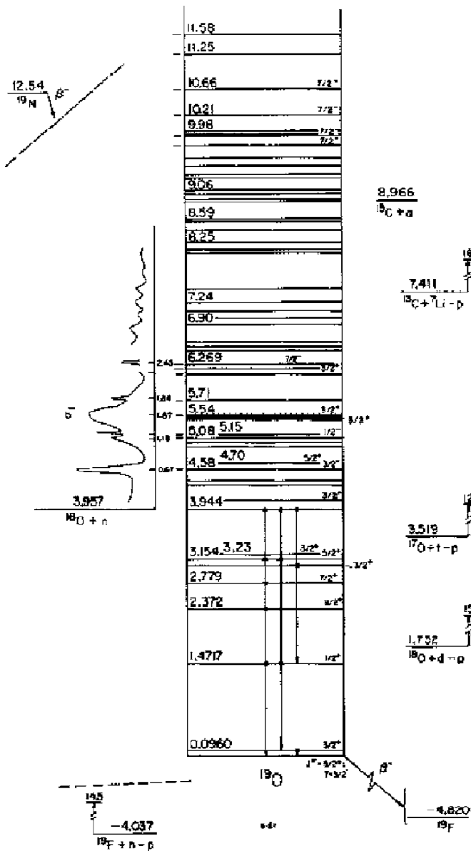
FIG. 1. The spectrum of ^{19}\text{O} . From Ajzenberg-Selove, 1987 .
