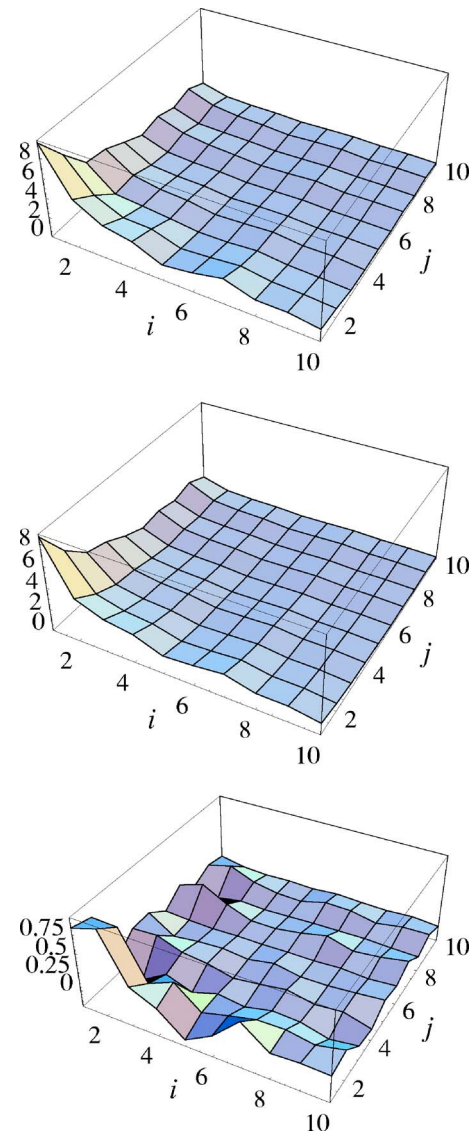
FIG. 20. (Color online) Same as Fig. 18 except for the correlations between pairs of nearest-neighbor spacings of low-lying levels with different spins obtained by averaging over a number of nuclei in the sd shell (see text). The indices i and j label the spacings consecutively starting from the lowest state. Left panel: Mean value of the product of the two spacings. Middle panel: Product of the mean values of the two spacings. Right panel: The correlator. From Papenbrock and Weidenmüller, 2006.
