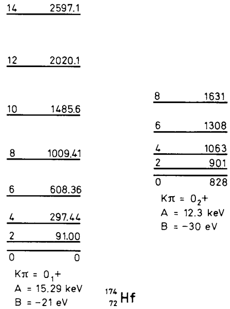
FIG. 2. Rotational bands in ^{174}\text{Hf} . From Bohr and Mottelson, 1975 .
