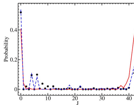
FIG. 16. (Color online) Six fermions in the j=19/2 shell with 900 realizations of the TBRE. Solid line: Numerical probabilities for \sigma_J to have maximum value. Dashed line: Numerical probabilities for r_J \sigma_J to have maximum value. Dots: Numerical probabilities for state with spin J to be the ground state. From Papenbrock and Weidenmüller, 2004.
