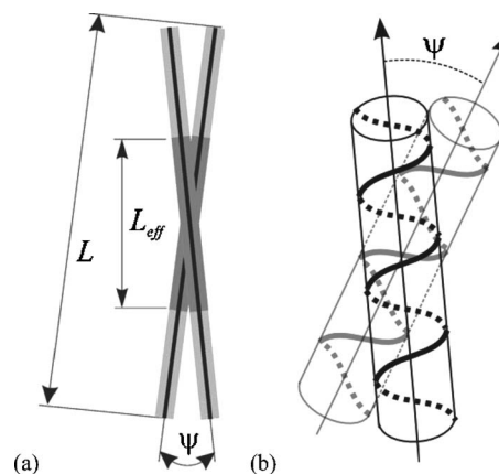
FIG. 12. Schematic illustration of two helices skewed at an angle of \psi . (a) The length of effective juxtaposition ( L_{eff} ) represents the region of significant overlap between electric fields created by molecules, which determines the electrostatic interaction energy. (b) Relative orientation of strands and grooves within the effective juxtaposition region determines the chiral torque between molecules. The helix with lighter markings lies behind that with darker markings. As shown here, right-handed helices prefer a right-handed twist to prevent crossing of the helical strands (dashed dark lines on the back of the front helix and solid gray lines on the front of the helix in the rear). For cholesteric liquid crystals, such a preferred twist will result in a right-handed cholesteric chirality. In the case of supercoils (or coiled coils), this preferred twist will yield a left-handed supercoil since such a twist will lead to helices wrapping around each other in the chiral sense opposite to their own handedness.
