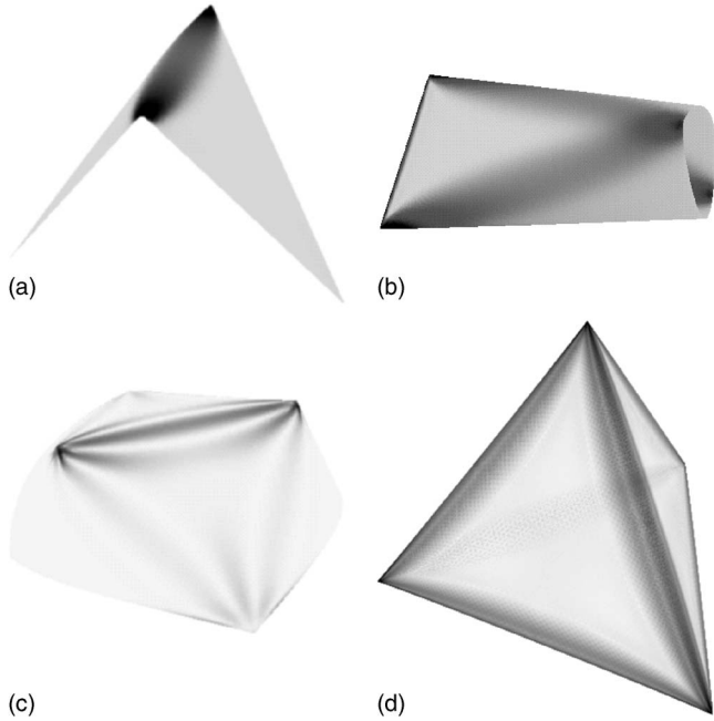
FIG. 11. Simulated configurations showing ridge scaling: kite, bag, boat, after Lobkovsky et al. (1995). Kite construction is explained in Fig. 12. The bag, boat, and tetrahedron are formed by removing sectors from a flat sheet of material and fastening the cut edges together, as implemented in Fig. 9. Shading is proportional to local stretching energy density. Alternating bright and dark stripes indicate nonmonotonic distribution of energy. The tetrahedron at the lower right (DiDonna, 2005) has h_c/X=10^{-4} and has a ratio of bending to stretching energy B/S=5.1 . The simulation has 80 lattice points along the ridge.
