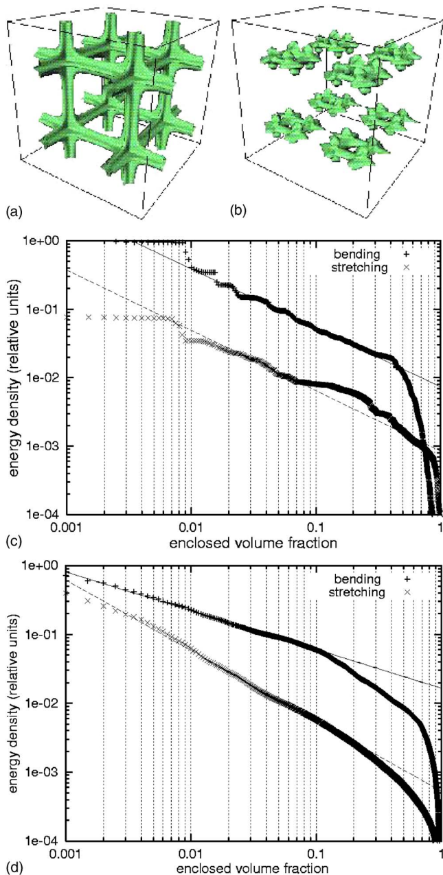
FIG. 15. (Color online) Energy density profiles for a simulated elastic cube with opposite faces joined to make a torus, embedded in four dimensions (a), (c) and five dimensions (b), (d), after DiDonna et al. (2002). Upper pictures show the material coordinates with 2.5% of the volume with highest density indicated. Log-log plots show the corresponding energy profiles. Upper curves are bending energy density; lower curves are stretching energy density.
