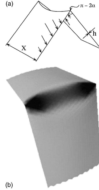
FIG. 13. Two views of the minimal ridge. (a) Sketch of the minimal ridge configuration. Normal forces needed to constrain the edges to the frame are indicated. Bending angle \alpha , thickness h , and ridge length X are indicated. The positive direction for f and for curvature is downward in this view. (b) Simulation with shading proportional to stretching energy density, after Lobkovsky and Witten (1997).
