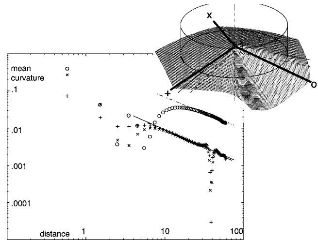
FIG. 10. Log-log plot of mean curvature along three radial lines of the d -cone shown in the inset, after Liang and Witten (2006) . Circles, line in the buckled region, indicated by the heavy line in the inset marked with \circ . + , \times , lines that touch the confining ring, indicated by heavy lines marked with + and \times .
