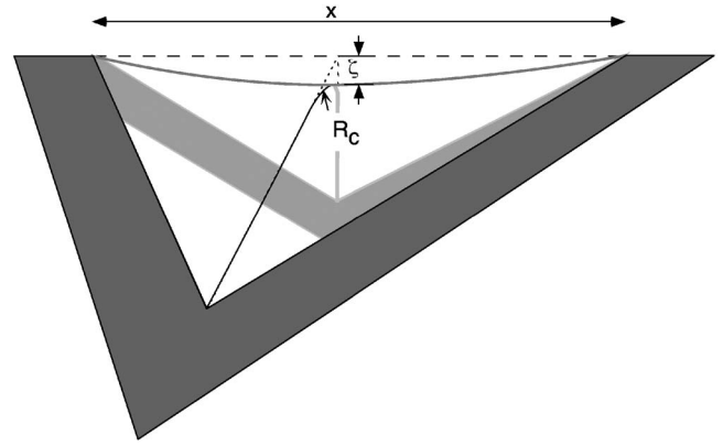
FIG. 12. The kite, a square of elastic material fastened in a hinged frame. Base line is shown as a dashed, horizontal line. The transverse midline goes from front to back. This line is the y axis of the material coordinates. The x axis is the ridge line. Ridge length X , assumed curvature radius R_c , and sag distance \zeta are indicated.
