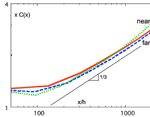
FIG. 14. (Color online) Log-log plot of normalized transverse curvature x C_{yy} near a vertex vs distance normalized x/h along a ridge direction of a cube, after DiDonna (2005). The three curves correspond to three different-sized cubes. Top curve at the right edge reaches the midpoint of the cube edge. Bottom curve reaches 1/10 of the distance to the midpoint. For an isolated vertex, x C_{yy} is independent of x . For a ridge, x C_{yy} is expected to scale as x^{1/3} .
