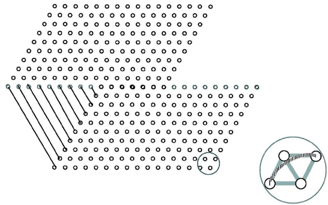
FIG. 9. (Color online) Lattice of springs to simulate an elastic sheet, after Seung and Nelson (1988). Inset at right shows nearest-neighbor springs (light lines) and spring between adjacent triangles to impart bending stiffness (dark line). One may make a disclination cone by removing a sector of the lattice and joining boundary particles with springs as shown by the lines at the lower left. If both sectors are joined in this way, the minimum-energy shape of the surface has the boat shape shown in Fig. 11. Inset to Fig. 10 shows a hexagonal section of a similar lattice deformed into a d -cone.
