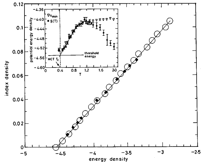
FIG. 12. Index density vs potential energy. Average over all data was obtained by sampling at T^* \in [0.3, 2.0] . The solid line is a linear fit meeting the energy axis at u_{\text{th}} (see text). Inset shows the average density of the local minima u_{\text{min}} as a function of the temperature of the initial MD trajectory. Circles represent \delta T , the average potential-energy density \langle U/N \rangle(T) less the vibrational energy 3T/2 in the harmonic approximation. The threshold energy u_{\text{th}} = -4.55 is reached at T^* = 0.44 \approx T_c (see text).
