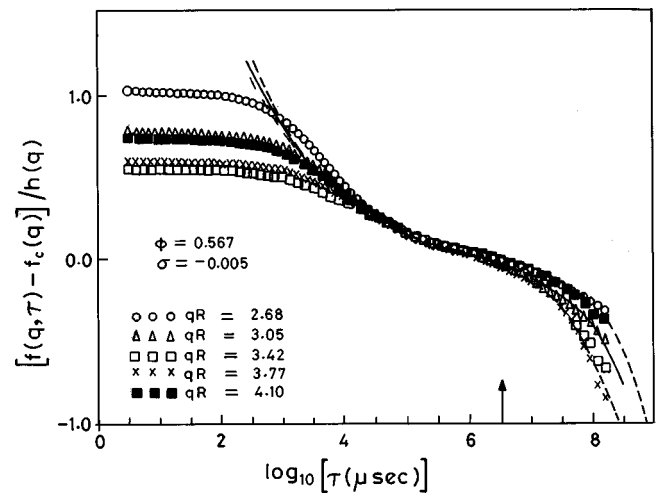
FIG. 9. The density correlator \phi_q(t) \equiv f(q, \tau) in scaled form [\phi_q(t) - f_q]/h_q vs time t = \tau/R , the hard-sphere radius, \sigma , the separation parameter; \phi , the packing fraction; solid line, the mode-coupling master function \sigma^{1/2}[g_-(t)] (see text) corresponding to exponent parameter \lambda=0.758 ; dashed lines, \lambda=0.70 and 0.80 , respectively. The vertical arrow on the time axis corresponds to the \beta relaxation time scale \tau_\beta . From van Megen and Underwood, 1994.
