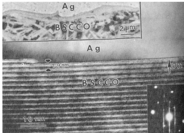
FIG. 66. High-resolution TEM image of an Ag-sheathed Ag-(Bi,Pb) _2 Sr _2 Ca _2 Cu _3 O _x tape. The SEM image shows the platelike phase at the Ag interface. From Feng et al. (1993); figure courtesy of Y. Feng and D. C. Larbalestier, University of Wisconsin, USA.
