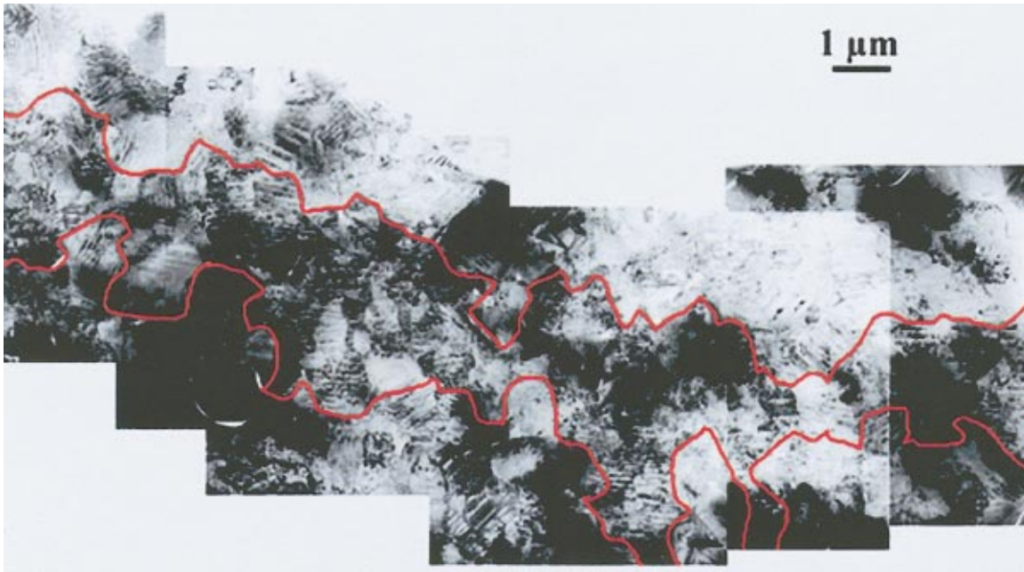
FIG. 69. Low-magnification, TEM-image montages depicting the colony structures of well-aligned grains in a 1- \mu m -thick YBa_2Cu_3O_{7-\delta} film grown by pulsed laser deposition on a polycrystalline Ni-based substrate. The linkage of the colonies, shown by the outlined regions, provides a percolation pathway for the transport supercurrent. From Kung et al. (1999); figure courtesy of H. Kung, Los Alamos National Laboratory, USA [Color].
