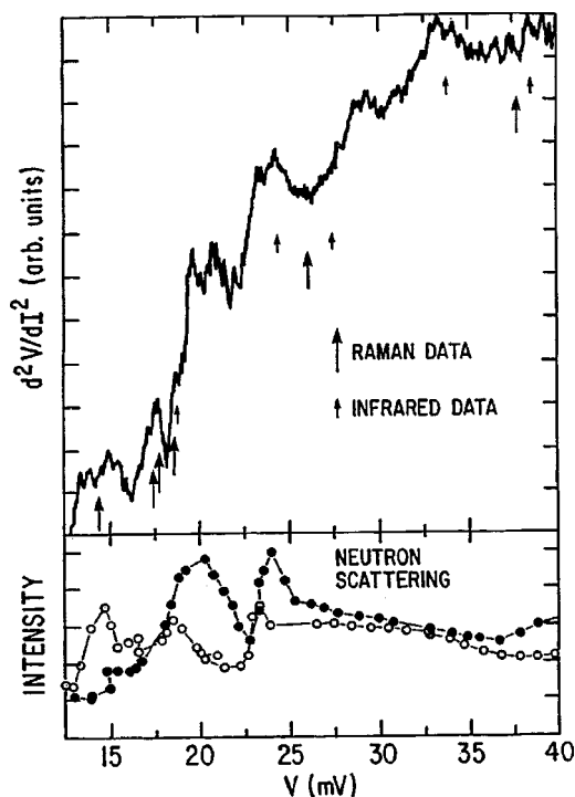
FIG. 24. The second derivative, d^2V/dI^2 , of the I(V) characteristic of a 45^\circ [001]-tilt grain-boundary junction in a \text{YBa}_2\text{Cu}_3\text{O}_{7-\delta} film measured at 4.2 K. Shown for comparison are phonon data obtained by other techniques; the larger arrows indicate the positions of Raman lines, the smaller arrows infrared reflection lines and inelastic neutron data. From Chaudhari et al. , 1993; figure courtesy of P. Chaudhari and E. Sarnelli, IBM T.J. Watson Research Center, USA.
