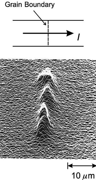
FIG. 63. Image of the voltage response signal of a 38° [001]-tilt grain boundary in a bicrystalline YBa 2 Cu 3 O 7- \delta film obtained by low-temperature scanning electron microscopy. The 20- \mu m-wide and 0.5- \mu m-thick bridge crossing the grain-boundary was biased at 14 K with a current of 39 mA. The signal images the voltage state of the grain boundary, which shows up because the bias current exceeds the critical current of the grain boundary but not of the grains. After Mannhart, Gross, et al. (1989).
