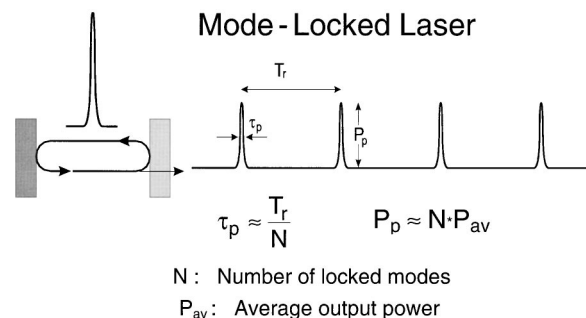
FIG. 2. Radiation power as a function of time at the output of a stationary mode-locked laser.
