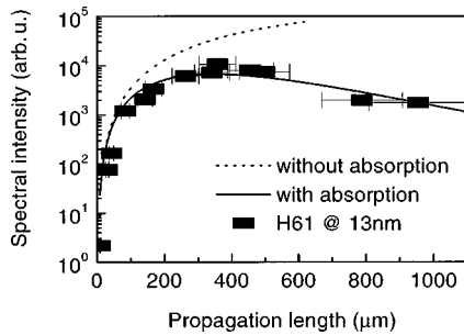
FIG. 37. Evolution of the 61st harmonic upon propagation of a few-cycle laser pulse in a neon target (300 Torr): ■, measured; solid curve, computed; dotted curve, result of the same calculation in the absence of absorption loss, \alpha=0 . The laser parameters are \lambda_0=0.8\ \mu\text{m} , I_0=5\times 10^{14}\ \text{W}/\text{cm}^2 , and \tau_p=5\ \text{fs} . The error bars result from uncertainties in estimating effective interaction lengths and the pressure in the interaction region. The computed data are multiplied by a constant scaling parameter yielding best agreement between experiment and theory (Schnürer et al. , 1999b).
