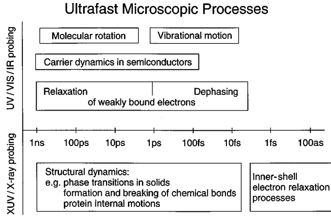
FIG. 50. Characteristic time scales of some elementary atomic, molecular, and collective processes. The boundaries of the presented time range are not intended to imply upper or lower limits on some of the processes.
