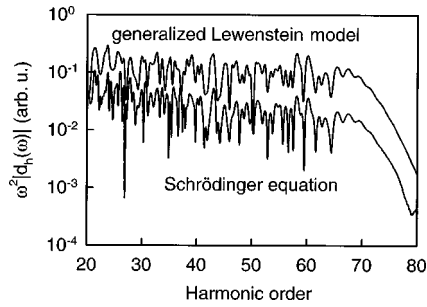
FIG. 36. Fourier transform of the single-atom dipole acceleration \omega^2|\tilde{d}_h(\omega)| for high harmonic generation in hydrogen as determined by solving Eqs. (34)–(39) and the time-dependent nonrelativistic Schrödinger equation. The laser electric field is determined by Eq. (33) and the laser parameters are I_0=5 \times 10^{14} W/cm 2 , \varphi_0=0 , \lambda_0=0.8 \mu\text{m} , and \tau_p=5 fs.
