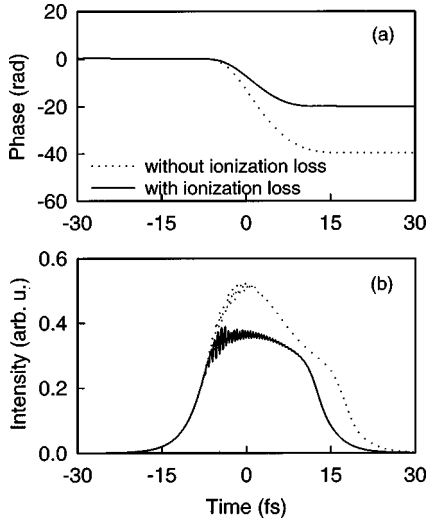
FIG. 28. A frequency-doubled Ti:sapphire laser pulse ( \lambda_0 = 0.4 \mu\text{m} ) after a propagation distance of 8 mm in helium (500 Torr): (a) Phase; (b) intensity envelope for the following laser parameters: I_0 = 2 \times 10^{15} \text{ W/cm}^2 , \tau_p = 10 \text{ fs} . Dotted curve, the solution of the wave Eq. (31), in one space dimension without the ionization-loss term; solid curve, solution with the ionization-loss term. Ionization loss appears to have a strong influence on the evolution of a few-cycle laser pulse. Because more electrons are ionized at the peak of the pulse than in the pulse wings, the ionization loss leads to a stronger reduction of the pulse peak and hence, to lengthening of the pulse. As a result the nonlinear interaction saturates faster and the blue-shifting and spectral broadening of the pulse is reduced. The observed behavior has important implications for strong-field phenomena, such as a modification of the effective interaction length for x-ray lasing and high harmonic generation.
