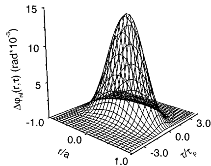
FIG. 14. Self-phase-modulation-induced phase \Delta\varphi_{nl}(z, r, \tau) imposed by the Kerr nonlinearity on a pulse in a hollow waveguide as a function of the radial and the temporal coordinates under conditions described in the caption of Fig. 13 for a propagation length of z=L_2/50 (Tempea and Brabec, 1998b). For z \ll L_2 , the signals coupled into different higher-order modes are comparable; therefore all coupling channels must be taken into account, resulting in a spatially varying phase shift that follows the transverse intensity profile of the fundamental \text{LP}_{01} mode. For pulse peak powers p_0 approaching p_{c,wg} , this phenomenon causes self-focusing of the beam, destroying propagation in the fundamental mode.
