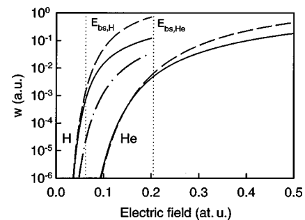
FIG. 31. Static field ionization rates in hydrogen and helium atoms vs the electric-field strength in atomic units: solid curve, numerical result; dashed curve, Ammosov-Delone-Krainov formula; dash-dotted curve, Keldysh theory for hydrogen. The dotted line denotes the barrier suppression field strength for H and He.
