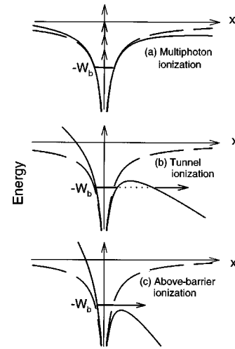
FIG. 30. Regimes of atomic ionization. Exposing an atom to an intense laser field will result in a modified potential (solid curve) composed of the Coulomb potential (dashed curve) and the time-dependent effective potential of the optical pulse. (a) At moderate intensities the resulting potential is close to the unperturbed Coulomb potential and an electron can be liberated only upon simultaneous absorption of N photons, resulting in multiphoton ionization. The multiphoton ionization rate scales with the N th power of the intensity of the optical pulse. (b) At sufficiently high field strengths the Coulomb barrier becomes narrow, allowing optical tunneling ionization to take over and resulting in a tunneling current that follows adiabatically the variation of the resultant potential. (c) At very high field strengths, the electric field amplitude reaches values sufficient to suppress the Coulomb barrier below the energy level of the ground state, opening the way to above-barrier ionization.
