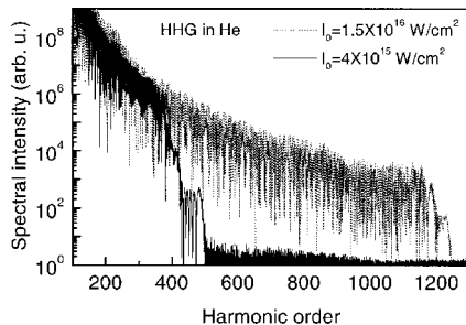
FIG. 43. Harmonic intensity spectra generated in a helium gas target at a gas pressure of 500 Torr after an interaction length of 125 \mu\text{m} for two different peak intensities: solid curves, I_0 = 4 \times 10^{15} \text{ W/cm}^2 ; dotted curve, I_0 = 1.5 \times 10^{16} \text{ W/cm}^2 . The remaining laser pulse parameters are \tau_p \approx 5 \text{ fs} and \lambda_0 \approx 0.8 \mu\text{m} .
