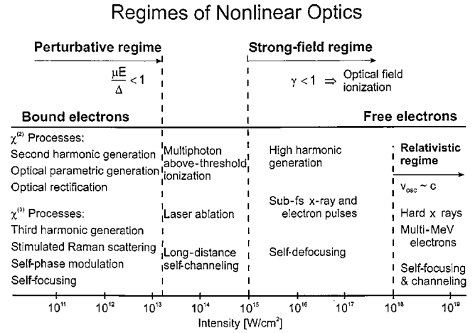
FIG. 24. Regimes of nonlinear optics. Only nonresonant interactions have been considered by assuming the detuning \Delta\hbar to be larger than the photon energy ( \approx 1 eV). The boundaries between different regimes are not sharply defined. In the strong-field regime, the intensity scale applies to the visible and near-infrared spectral range.
