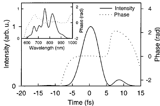
FIG. 19. Millijoule-scale pulses exiting the hollow-fiber chirped-mirror compressor: solid curve, intensity envelope; dotted curve, phase, with \varphi_0 chosen arbitrarily to be equal to zero; inset, spectrum. The data were retrieved from a frequency-resolved optical gating measurement (Cheng et al. , 1999). The pulse duration evaluated is \tau_p = 5.3 fs.
