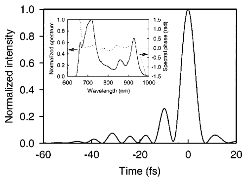
FIG. 17. Spectral intensity and phase (insert) and intensity envelope of sub-6-fs pulses produced by a semiconductor-saturable-absorber-initiated Kerr-lens mode-locking mirror-dispersion-controlled Ti:S laser (Sutter et al. , 1999). The data have been evaluated from a SPIDER (spectral phase interferometry for direct electric-field reconstruction) measurement (Gallmann et al. , 1999).
