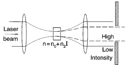
FIG. 5. Self-focusing-induced changes in the transmittivity of an aperture: the ultrafast-response saturable-absorber effect results in Kerr-lens mode locking.
