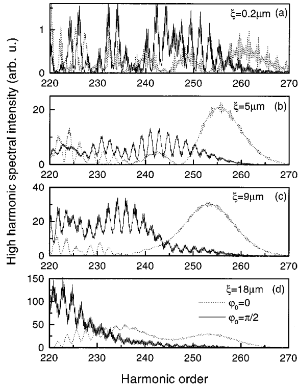
FIG. 48. Spectral intensity of the harmonic radiation in helium at a pressure of 500 Torr for the fundamental pulse phases: dotted curve, \varphi_0=0 ; solid curve, \varphi_0=\pi/2 , after propagation distances of (a) 0.2, (b) 5, (c) 9, and (d) 18 \mu\text{m} . The laser parameters are I_0=2\times 10^{15}\text{ W/cm}^2 , \lambda_0=0.8\text{ }\mu\text{m} , and \tau_p=5\text{ fs} . The electric field is defined by Eq. (33).
