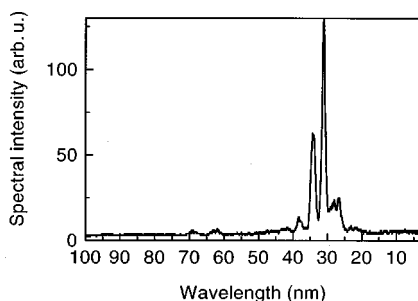
FIG. 38. Spectral harmonic intensity vs wavelength as generated in argon (300 Torr, interaction distance 2 mm). The laser parameters are \lambda_0=0.8\ \mu\text{m} , I_0=5\times 10^{14}\ \text{W}/\text{cm}^2 , and \tau_p=5\ \text{fs} .
