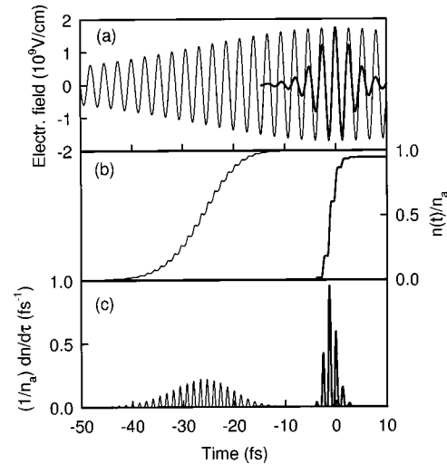
FIG. 32. Helium in the presence of a linearly polarized electric field of a laser pulse with \lambda_0 = 0.8 \mu\text{m} and a peak intensity I_0 = 4 \times 10^{15} \text{ W/cm}^2 : (a) electric field; (b) fraction of ionized electrons; (c) instantaneous ionization rate. The thin and the heavy lines represent pulses of durations of \tau_p = 50 \text{ fs} and \tau_p = 5 \text{ fs} , respectively.
