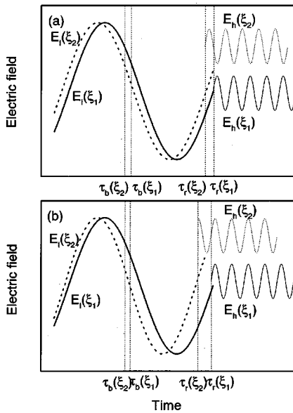
FIG. 40. Schematic of the laser field E_l and of the harmonic field E_h : solid curves, generated at \xi_1 ; dotted curves, generated at \xi_2 , in the limit of (a) adiabatic evolution of a many-cycle laser pulse and (b) nonadiabatic evolution of a few-cycle laser pulse; the coordinate frame is moving with c , the approximate phase velocity of the harmonic wave. In this frame, the harmonic field remains unchanged with propagation and the laser field changes only due to the free-electron-induced phase mismatch. For comments see the text.
