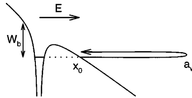
FIG. 25. Resultant (quasistatic) potential felt by the most weakly bound electron in the presence of a strong laser field. The electron can tunnel through the barrier. It is born at the position x_0 with some drift velocity (Corkum et al. , 1989) and follows the periodic motion of the laser field. The maximum amplitude during the first excursion is denoted by a_w .
