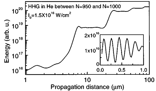
FIG. 44. Energy of the harmonic signal integrated between N=950 and N=1000 vs propagation distance for the parameters of Fig. 43 ( I_0 = 1.5 \times 10^{16} \text{ W/cm}^2 ). The inset shows the growth of the harmonic over the first \mu\text{m} .
