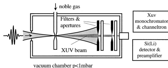
FIG. 33. Schematic of the experimental setup of a typical high harmonic generation experiment. The laser beam is focused into the target chamber. The target is formed by a tube, in whose walls are holes bored by the laser itself. The tube is continuously backed with some noble gas. The generated high harmonic radiation is measured either by wavelength-dispersive spectral analysis or by energy-dispersive x-ray spectrometry (courtesy of Ch. Spielmann).
