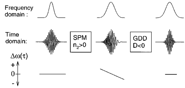
FIG. 11. Schematic representation of optical pulse compression. The graphs depict qualitatively the spectral intensity distribution (frequency domain), and evolution of the electric field E(t) and change in instantaneous frequency with respect to the carrier frequency \Delta\omega(\tau) = \omega_{\text{inst}}(\tau) - \omega_0 (time domain). The bandwidth-limited [ \Delta\omega(\tau) = 0 ] input pulse propagates from the left to the right. The positive frequency sweep \Delta\omega(\tau) = (d/d\tau)\Delta\varphi_{nl}(\tau) imposed on the intense light pulse by self-phase-modulation induced by the optical Kerr effect upon passage through a transparent optical medium can be removed by subsequently passing the pulse through a dispersive delay line with negative group delay dispersion, resulting in a temporal compression.
