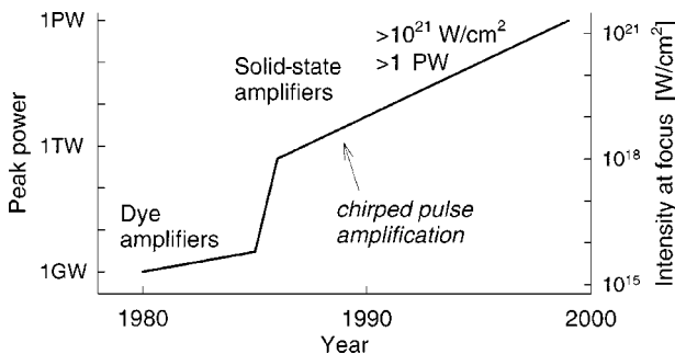
FIG. 8. Evolution of ultrashort-pulse amplification in terms of peak power and achievable peak intensity.
