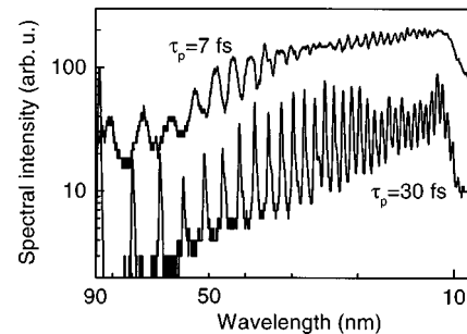
FIG. 35. Harmonic spectra generated in neon at a pressure of 250 Torr for Ti:sapphire laser pulses of 30 and 7 fs (FWHM) carried at \lambda_0 \approx 0.8 \mu\text{m} . The peak intensity of both pulses was \approx 3 \times 10^{14} \text{ W/cm}^2 . At the peak of the 30-fs pulse roughly 10% of the neon atoms are ionized, while at the peak of the 7-fs pulse 1% are ionized (courtesy of M. Schnürer).
