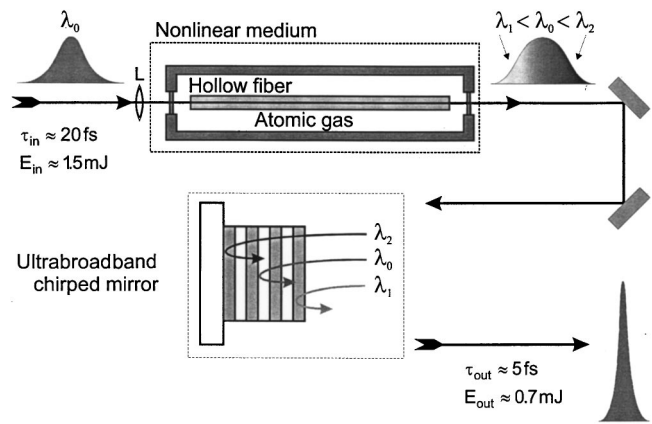
FIG. 16. Schematic experimental setup of a hollow-fiber chirped-mirror high-energy pulse compressor. The input pulse is coupled into a gas-filled hollow fiber, where its spectrum is broadened by self-phase-modulation imposed by the optical Kerr effect in the gas. Subsequently, the chirp of the broadened pulse is removed upon reflection off broadband chirped mirrors [see diagrams (a) and (b) in Fig. 10], which leads to a temporal compression of the laser pulse (courtesy of A. Poppe).
