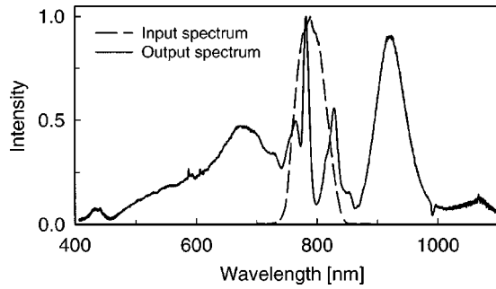
FIG. 18. Typical spectrum before (dashed line) and after (solid line) propagation through a hollow fiber having a channel diameter of 250 \mu\text{m} and a length of approximately 1 m. The waveguide is seeded with 25-fs, 1.5-mJ input pulses and filled with neon at a pressure of \approx 1 bar.
