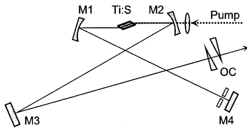
FIG. 15. Schematic of a mirror-dispersion-controlled Ti:sapphire laser made up of chirped mirrors (M1-M4), a broadband output coupler (OC), and a thin, highly doped Ti:sapphire crystal (Ti:S); for more details see, for example, Xu et al. (1997).
