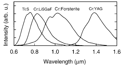
FIG. 4. Fluorescence emission spectra of some transition-metal-doped broadband solid-state laser crystals.
