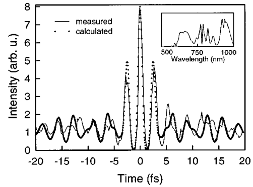
FIG. 20. Intense pulses originating from double-stage pulse compression, as described in the text and reported by Cheng et al. (1998): solid curve, measured interferometric autocorrelation; dotted curve, calculation from the inverse Fourier transform of the measured spectrum in the absence of a frequency-dependent phase, yielding a FWHM pulse duration of \tau_p = 4 fs; inset, spectrum.
