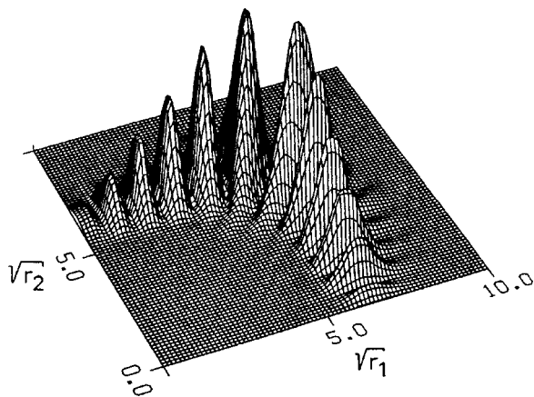
FIG. 18. The (m, l, k) = (5, 0, 0) wave function (projected onto \Theta = \pi ) in {}^3S^e helium; (N, K)_n = (6, 5)_6 ; the localization along the asymmetric stretch orbit [see Fig. 13(b)] is clearly visible (from Wintgen et al. , 1992).
