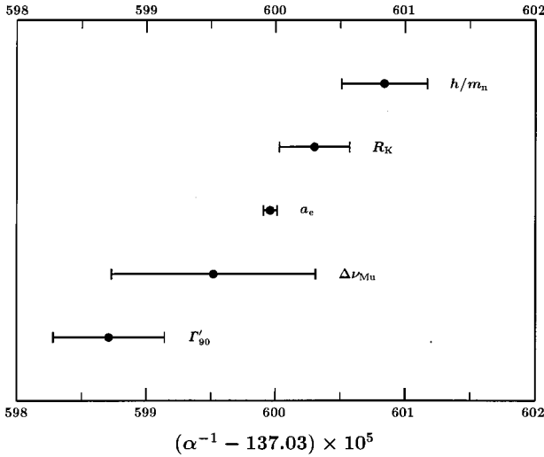
FIG. 3. Graphical comparison of the five values of the inverse fine-structure constant \alpha^{-1} given in Eqs. (352) to (356), in order of increasing value of \alpha^{-1} .
