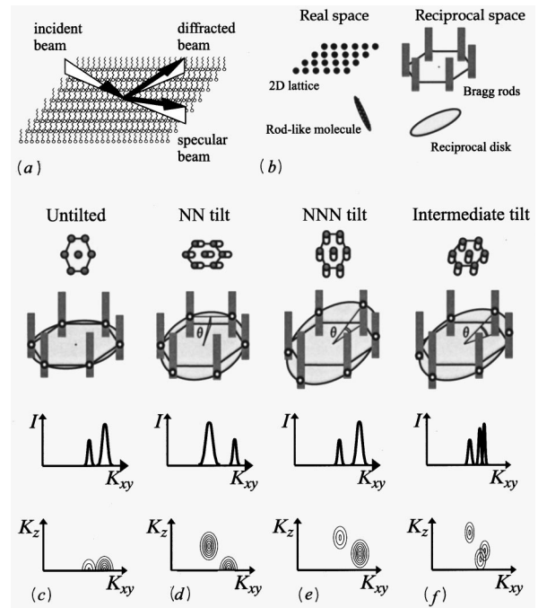
FIG. 5. X-ray-diffraction experiment: (a) schematic diagram of a grazing incidence x-ray-diffraction experiment; (b) formation of the diffraction pattern of a monolayer of rodlike molecules; (c) real-space and reciprocal-space views and characteristic diffraction patterns of the monolayer in untilted phase, (d) NN-tilted phase, (e) NNN-tilted phase, and (f) intermediate tilted phase (Kaganer et al. , 1995).
