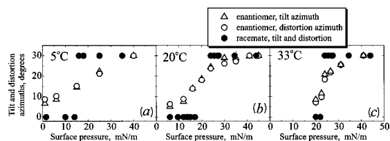
FIG. 25. Azimuth of tilt and that of the unit-cell distortion in a chiral monolayer of 1-hexadecyl-glycerol and in the racemic mixture of its left- and right-hand enantiomers (Scalas et al. , 1996, 1998). The nonchiral racemic monolayer experiences a first-order transition from NN to NNN tilt, while the chiral monolayer of the enantiomer undergoes a continuous variation of the tilt azimuth from a state close to the NN tilt to the one close to the NNN tilt. The azimuth variation becomes steeper with increasing temperature.
