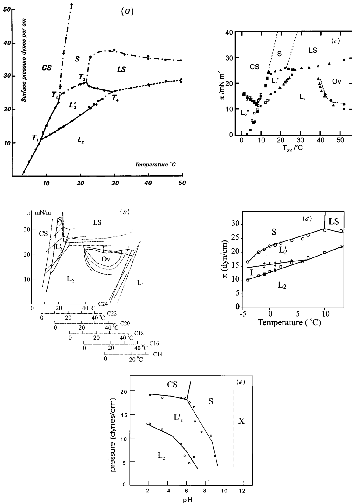
FIG. 3. Phase diagrams of fatty acid monolayers: (a) behenic ( \text{C}_{22} ) acid (Ställberg-Stenhagen and Stenhagen, 1945); (b) \text{C}_{14} – \text{C}_{24} acids. Adapted from Peterson et al. (1992), with data by Overbeck and Möbius (1993) added to locate the relative positions of the \text{C}_{16} – \text{C}_{20} phase diagrams more precisely; (c) behenic ( \text{C}_{22} , squares) and arachidic ( \text{C}_{20} , triangles and diamonds) acids, the temperature for the \text{C}_{20} measurements has been shifted by -10\text{ K} to overlay the \text{C}_{22} data (Rivière et al. , 1994); (d) arachidic ( \text{C}_{20} ) acid, showing an intermediate tilted phase (Durbin et al. , 1997); (e) heneicosanoic ( \text{C}_{21} ) acid with calcium ions in the subphase (Shih et al. , 1992b).
