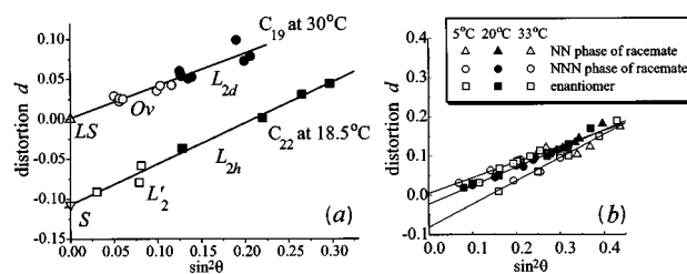
FIG. 12. The unit-cell distortion versus \sin^2 \theta : (a) fatty acids (data from Kenn et al. , 1991 and Durbin et al. , 1994); (b) a chiral substance 1-hexadecyl-glycerol (Scalas et al. , 1996, 1998). At a given temperature, different phases contribute to a common regression line, confirming the commonality of the structures.
