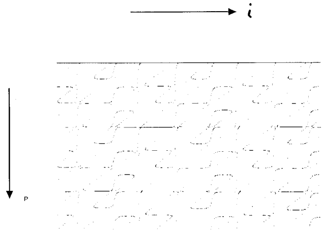
FIG. 48. Close-returns plot \Theta(\epsilon - |x(i) - x(i+p)|) of Belousov-Zhabotinskii data. Horizontal line segments indicate regions of data set that are near unstable periodic orbits.
