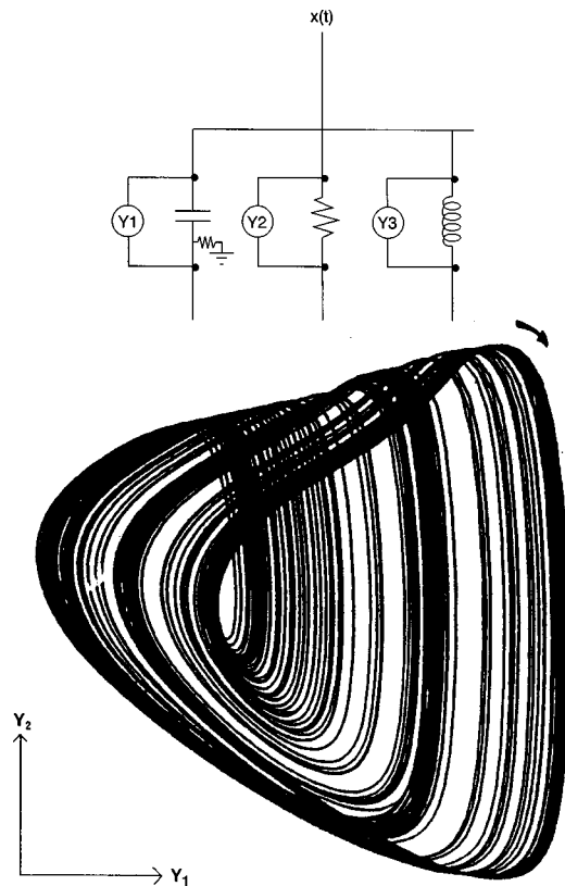
FIG. 57. Projection of the integral-differential phase-space embedding into the x - x plane. The integral is carried out with exponentially decreasing memory. Inset shows how this embedding can be carried out on-line.
