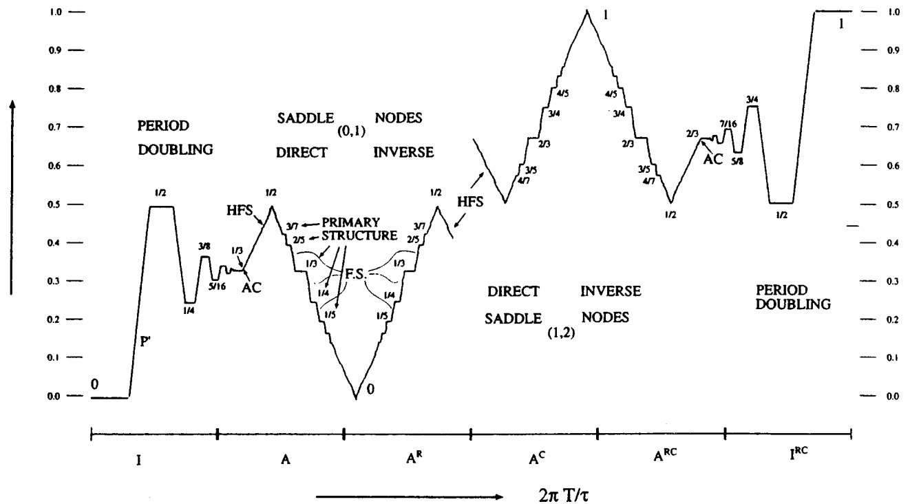
FIG. 83. Local torsion perestroika. Local torsion in a nonlinear oscillator changes in a systematic way as orbits are created on a direct horseshoe and annihilated from the reverse horseshoe.
