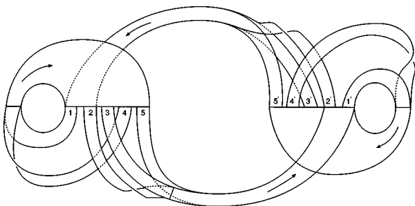
FIG. 19. One possible branched manifold for a flow.
