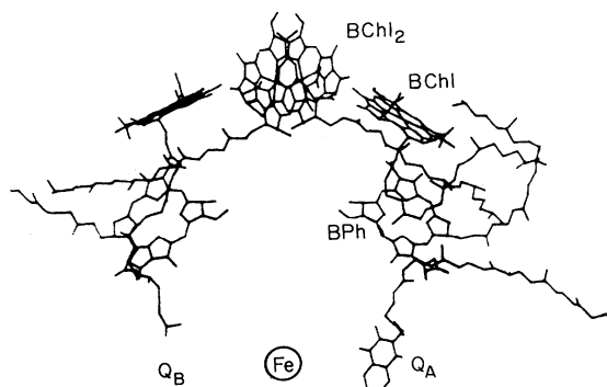
FIG. 11. Redox-active species involved in the initial charge separation for a photosynthetic bacterium (Deisenhofer et al. , Ref. 3; cf. Yeates et al. , Ref. 3), with labels added, to conform to the present text; they include a missing \text{Q}_B .
