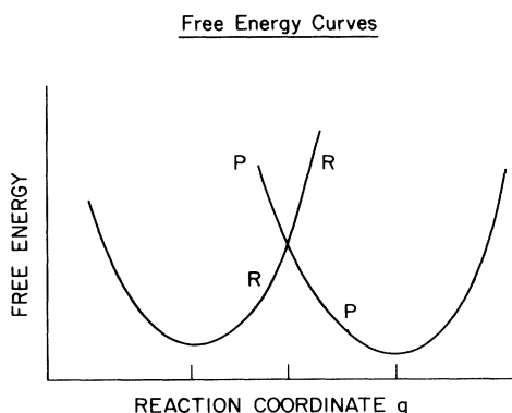
FIG. 5. Free energy of reactants plus environment vs the reaction coordinate q ( R curve), and free energy of products plus environment vs reaction coordinate q ( P curve). The three vertical lines on the abscissa denote, from left to right, the value for the reactants, for the transition state, and for the products (Marcus and Siddarth, Ref. 2).
