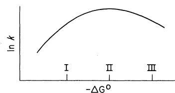
FIG. 7. Plot of \ln k , vs -\Delta G^0 . Points I and III are in the normal and inverted regions, respectively, while point II, where \ln k , is a maximum, occurs at -\Delta G^0 = \lambda (Marcus and Siddarth, Ref. 2).
