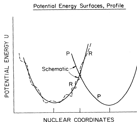
FIG. 4. Profile of potential energy surfaces for reactants plus environment, R , and for products plus environment, P . Solid curves: schematic. Dashed curves: schematic but slightly more realistic. The typical splitting at the intersection of U_r and U_p is not shown in the figure (Marcus and Siddarth, Ref. 2).
