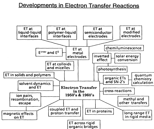
FIG. 1. Examples of topics in the electron transfer field (Marcus and Siddarth, Ref. 2).
