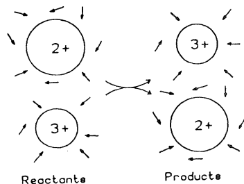
FIG. 3. Typical nuclear configurations for reactants, products, and surrounding solvent molecules in reaction (1). The longer M\text{-OH}_2 bond length in the +2 state is indicated schematically by the larger ionic radius (Sutin, Ref. 2).
