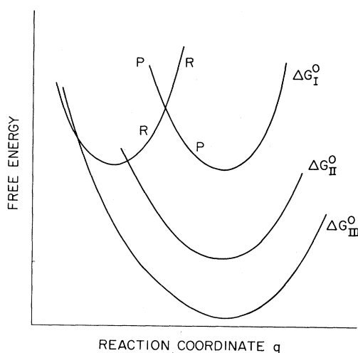
FIG. 6. Plot of the free energy G vs the reaction coordinate q , for reactants (R) and products (P), for three different values of \Delta G^0 , the cases I to III indicated in Fig. 7 (Marcus and Siddarth, Ref. 2).
