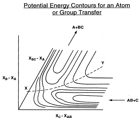
FIG. 2. Potential energy contours for reaction (4), AB + C \rightarrow A + BC , in the collinear case.
