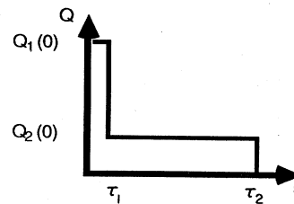
FIG. 4. Double step of relaxation.
