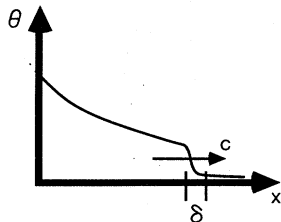
FIG. 2. Smoothing of a shock wave due to an effective conductivity, c=(k/\gamma\tau_1)^{1/2} , \delta=(k_1x/k)^{1/2} .
