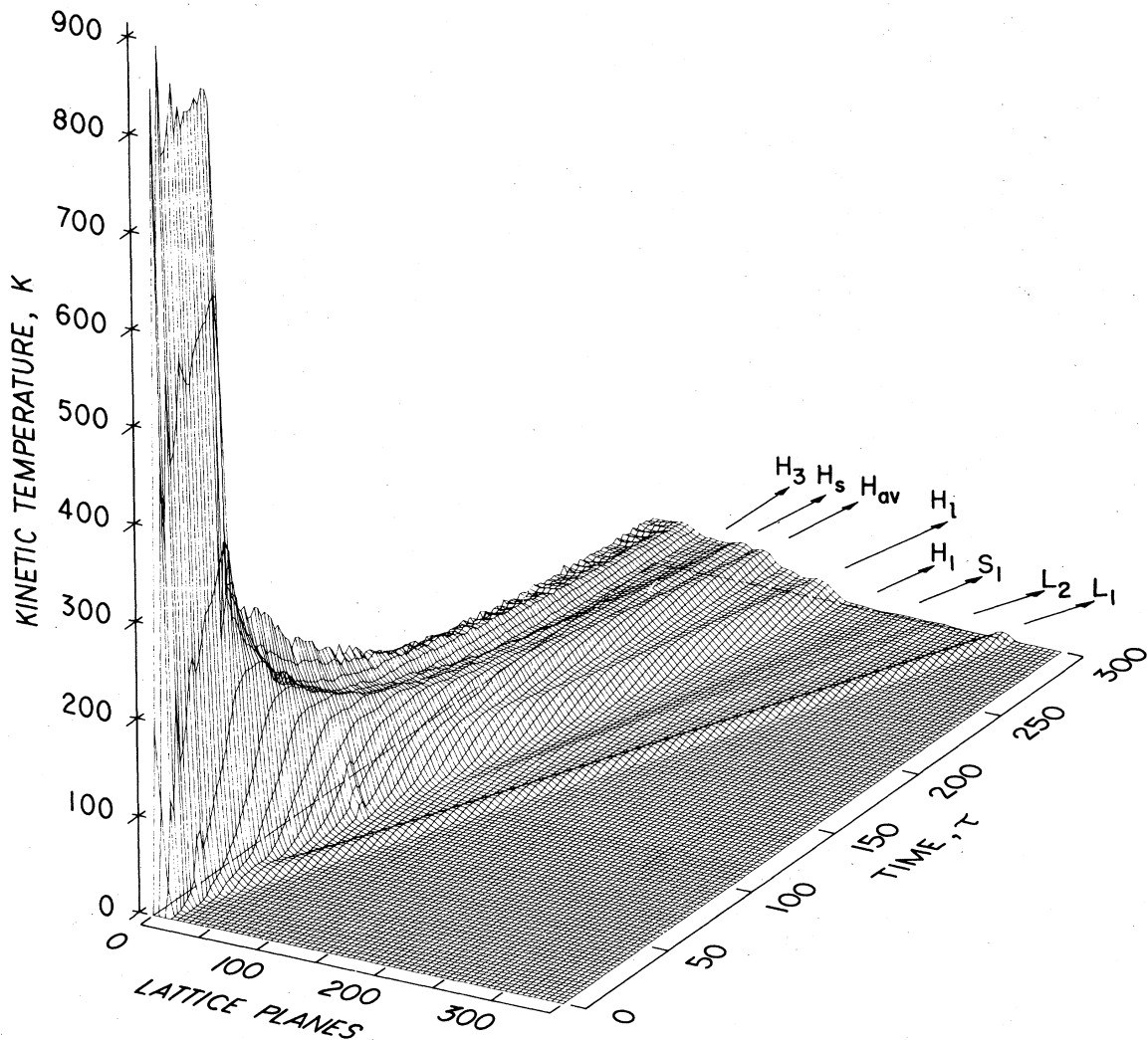
FIG. 5. Evolution of kinetic temperature profile K as a function of lattice plane number and time \tau for T_i = 0 K, mirror boundary conditions, and three-dimensional lattice. L_1 , L_2 , S_1 , H_1 , H_l , H_{av} , H_s , and H_3 label features in the profile moving with constant velocity. From Tsai and MacDonald, 1976.
