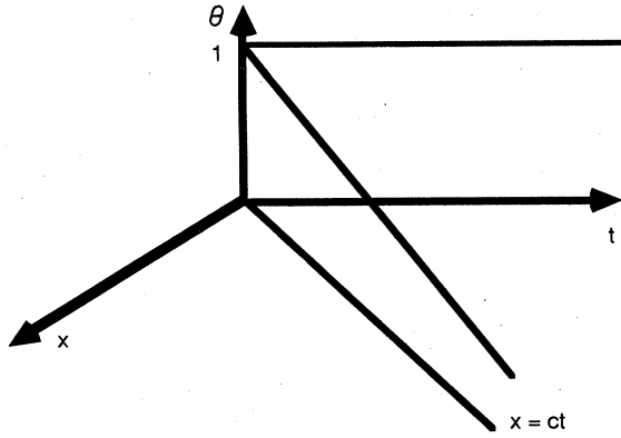
FIG. 1 Solution surface for Eq. (3.3) when \kappa_1=0 .
