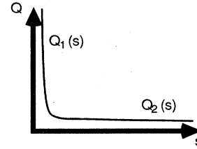
FIG. 3. Example of relaxation function with a fast and slow relaxation. The time \tau locates the end of the fast relaxation.
