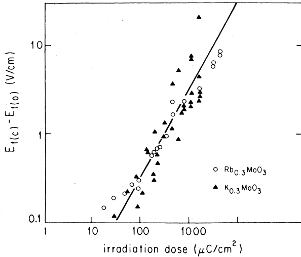
FIG. 21. Threshold electric field vs irradiation dose in K_{0.3}MoO_3 and Rb_{0.2}MoO_3 (from Mutka et al. , 1984).
