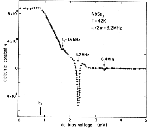
FIG 44. Real part of the ac conductivity \text{Re}\sigma(\omega) and dielectric constant \epsilon(\omega) measured at \omega/2\pi=3.2 MHz as a function of applied dc bias voltage. The threshold field is indicated by an arrow (Zettl and Grüner, 1984).
