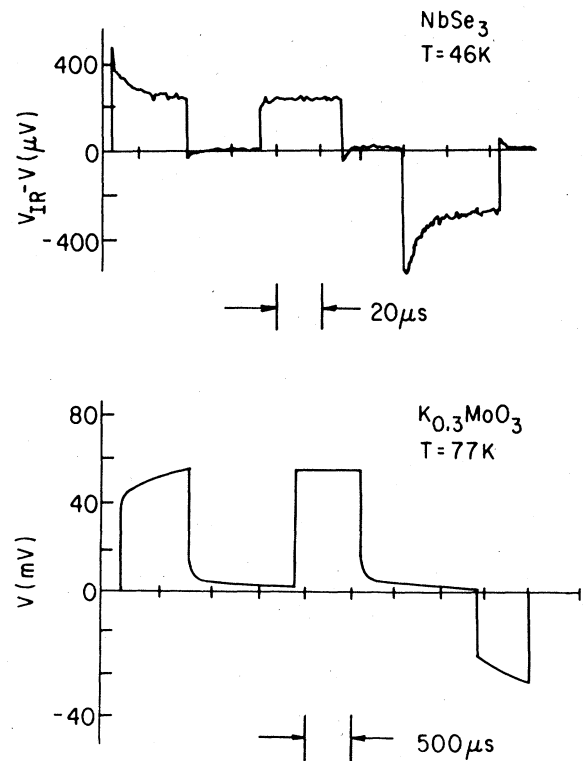
FIG. 53. Pulse sign memory effect. Response of NbSe 3 and K 0.30 MoO 3 to a repetitive series of constant-current pulses consisting of two positive pulses followed by one negative pulse. The amplitude of the pulses are in excess of threshold. When the current direction is reversed, the response becomes very slow. (a) for NbSe 3 ; the linear response is subtracted so that only IR_{\text{linear}} - V(t) is plotted as a function of time; (b) the total signal V(t) is plotted.
