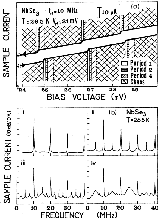
FIG. 49. (a) Schematic representation of the current response in the Shapiro step region of \text{NbSe}_3 , for forward and reverse bias voltage sweeps. The heavy lines are the direct I - V traces, offset vertically for clarity; (b) frequency spectrum of the current response in the Shapiro step region. External rf drive frequency and amplitudes as in (a). (i) V_{dc} = 25.0 mV, period 1; (ii) V_{dc} = 25.1 mV, period 2; (iii) V_{dc} = 25.2 mV, period 4; (iv) V_{dc} = 25.5 mV, chaos (Hall et al. , 1985).
