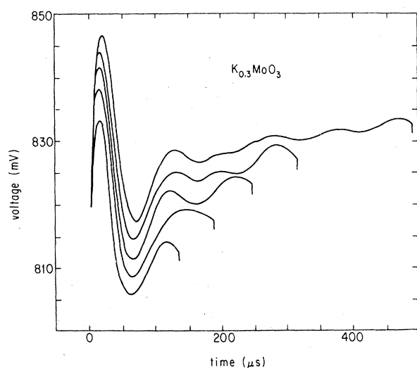
FIG. 54. Voltage response to repetitive pulse drive. For repetitive pulses of constant amplitude, the phase of the last transient oscillation is fixed relative to the end of the pulse for arbitrary pulse width (Fleming et al. , 1986).
