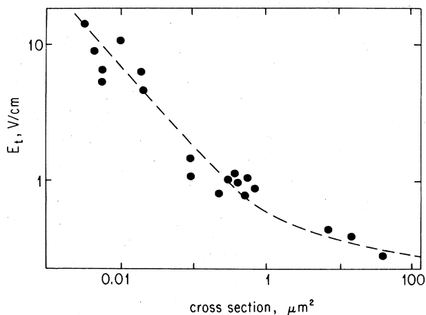
FIG. 24. Dependence of the threshold field E_T on the cross section of the specimens in the upper CDW state of NbSe 3 .
