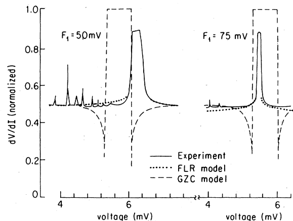
FIG. 48. Differential resistance dV/dI vs dc voltage V_0 near the first harmonic feature Q \cdot v \sim \omega_{ac} for NbSe 3 with ac frequency \omega_{ac}=25 MHz and ac voltage amplitudes V_1 \sim 50 and 75 mV (Brown and Grüner, 1988) for a sample with V_T \sim 2 mV. Also shown are theoretical fits using the Fukuyama-Lee-Rice (FLR) deformable CDW model (dotted line) and the Grüner-Zawadowski-Chaikin (GZC) one-degree-of-freedom result (dashed line). For FLR, both curves are fitted by use of a single parameter of order unity, as discussed in the text. The tops of the peaks are not calculated because the perturbation theory breaks down when the change in dV/dI is large (Coppersmith and Littlewood, 1986).
