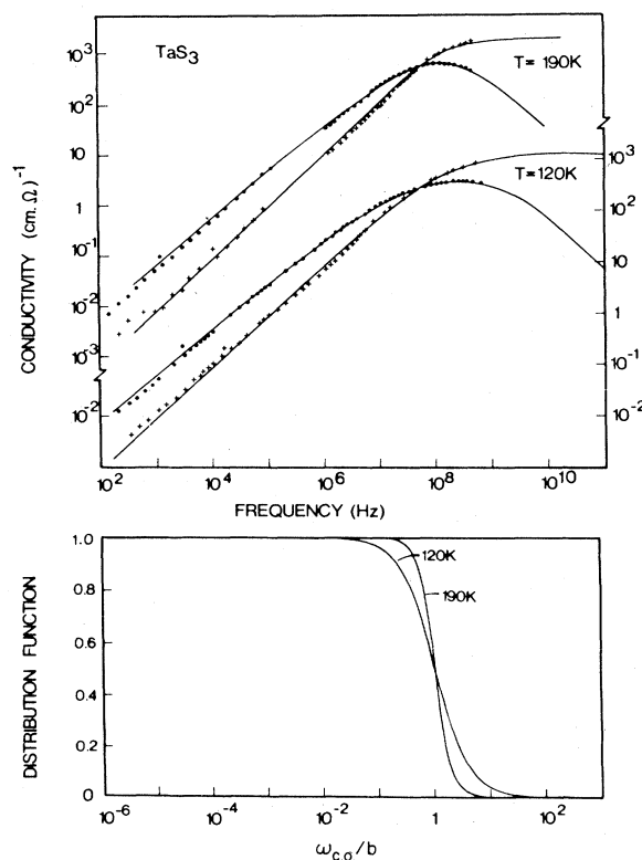
FIG. 31. Real and imaginary parts of the ac conductivity of \text{TaS}_3 vs frequency (Wu et al. , 1985).
