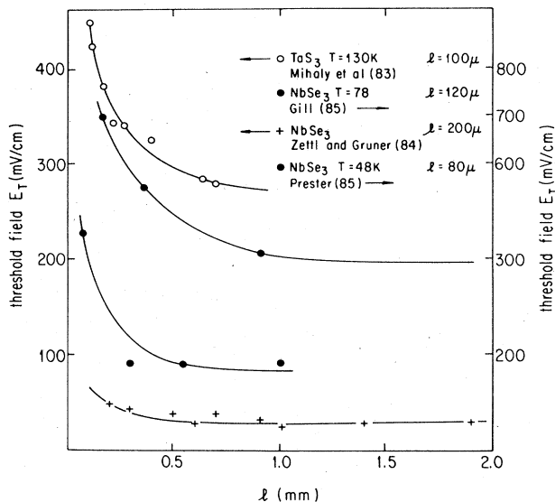
FIG. 23. Length dependence of the threshold field E_T in NbSe 3 and in TaS 3 . The solid lines are fits to Eq. (4.19) with L_0 values given on the figure.
