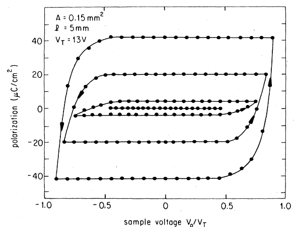
FIG. 52. Dielectric polarization loops observed in K_{0.3}MoO_3 at low temperatures. V_T refers to the threshold voltage for the onset of nonlinear conduction (Mihály and Tessema, 1986).
