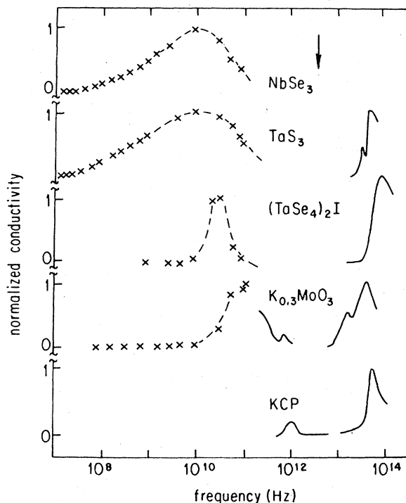
FIG. 9. The frequency-dependent conductivity of \text{NbSe}_3 , \sigma\text{-TaS}_3 and (\text{TaSe}_4)_2\text{I} , and \text{K}_{0.3}\text{MoO}_3 . The solid lines represent the regions where the drop signals the single-particle gaps; the strong peaks in the millimeter wave spectral range are due to the response of the pinned collective mode.
