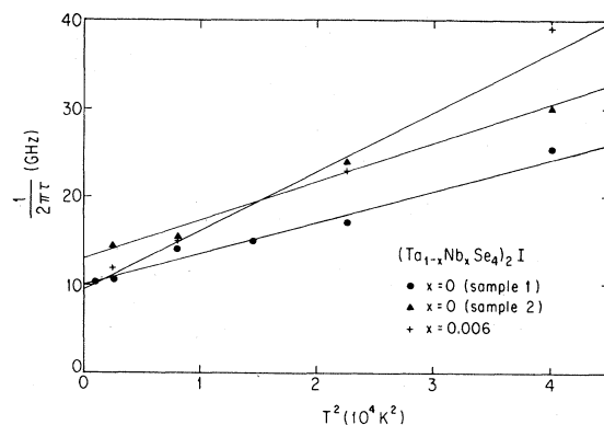
FIG. 30. Inverse relaxation time vs T^2 in two (\text{TaSe}_4)_2\text{I} specimens ( A and B ) and an alloy with 0.6% Nb. Samples A and B have a pinning frequency of \omega_0 = 17 and 35 GHz, respectively.
