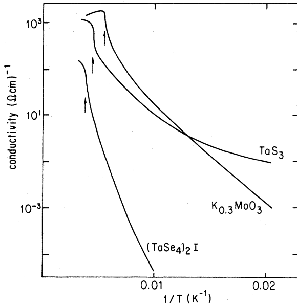
FIG. 4. Temperature dependence of the electrical conductivity in \sigma - \text{TaS}_3 , in (\text{TaSe}_4)_2\text{I} , and in \text{K}_{0.3}\text{MoO}_3 . The arrows represent the Peierls transition temperatures; they are evident by examining the temperature derivatives dR/dT .
