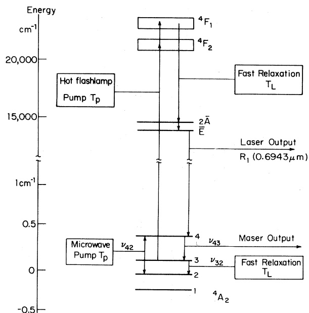
FIG. 2. Energy-level diagram of \text{Cr}^{3+} in ruby. Note change in vertical scale between microwave maser and optical laser action.
