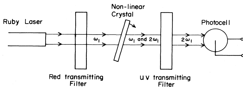
FIG. 3. Second harmonic generation of light.
