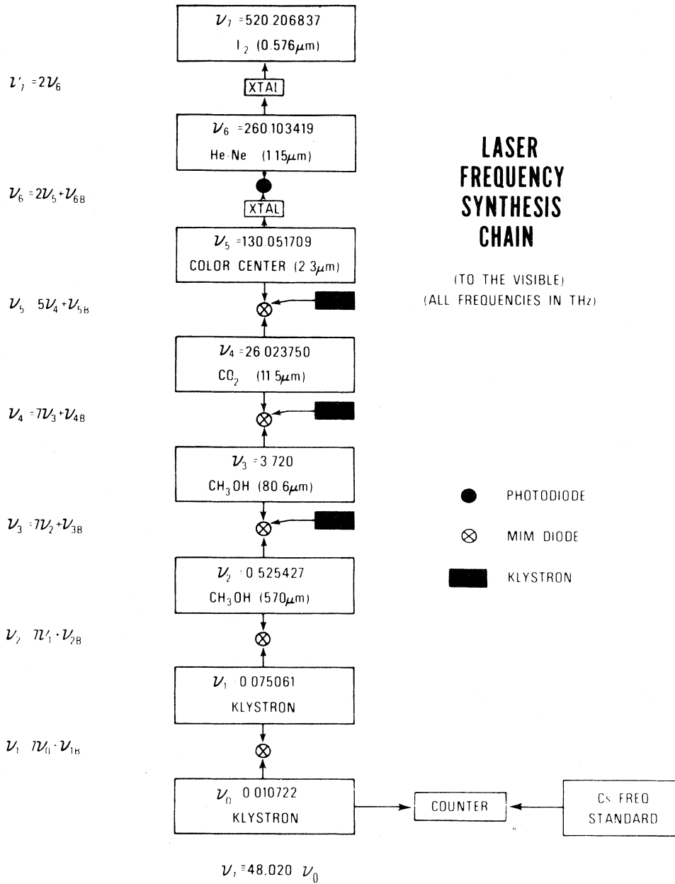
FIG. 6. Laser frequency synthesis chain (after Jenning, Petersen, and Evenson, 1979).
