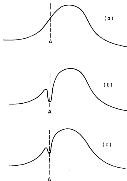
FIG. 1. (a) Inhomogeneous broadened profile of NMR in water. (b) Saturation dip in inhomogeneous profile, observed in 1946. (c) As in (b), but with longer delay between pump signal and probing scan. (after Bloembergen, Purcell, and Pound, 1948).
