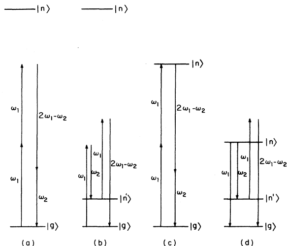
FIG. 8. The creation of a new beam at 2\omega_1 - \omega_2 by two incident beams at \omega_1 and \omega_2 , respectively, according to the geometry of Fig. 7(b). (a) Nonresonant mixing. (b) Intermediate Raman resonance (coherent anti-Stokes Raman scattering, or CARS). (c) Intermediate two-photon absorption resonance. (d) One-photon resonantly enhanced CARS.
