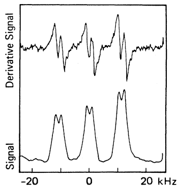
FIG. 5. High-resolution ( < 1 kHz) saturation spectroscopy of a ^{12}\text{CH}_4 spectral line near 3.39 \mu\text{m} wavelength. Each of the three hyperfine components is split into a doublet from the optical recoil effect. The upper curve is the experimental derivative trace (after Hall, Bordé, and Uehara, 1976).
