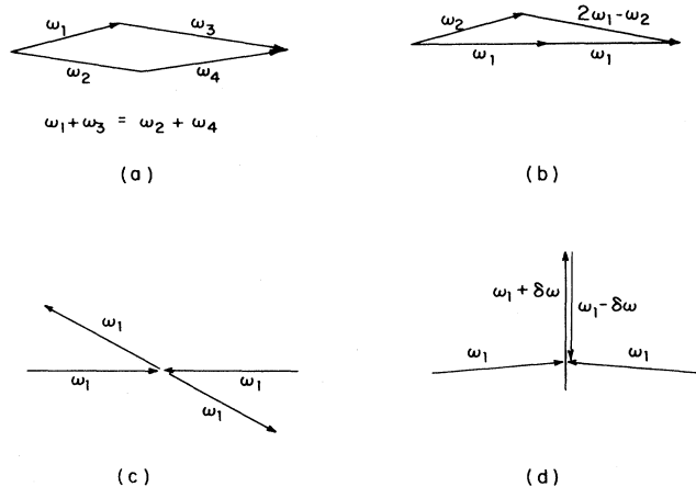
FIG. 7. Some typical wave-vector geometries of four-wave light mixing.
