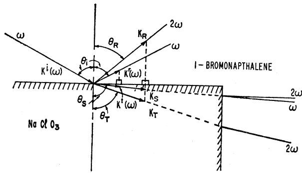
FIG. 4. Wave vectors of fundamental and second harmonic light waves at the boundary of a cubic piezoelectric crystal immersed in an optically denser fluid.
