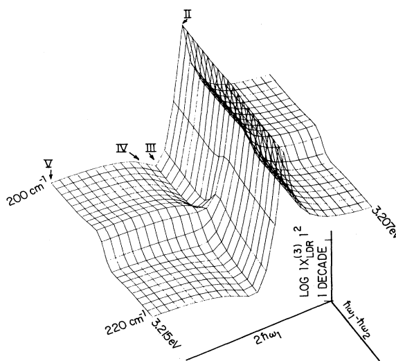
FIG. 9. Two-dimensional frequency dispersion of the nonlinear susceptibility \chi^{(3)} in cuprous chloride (after Kramer and Bloembergen, 1976).
