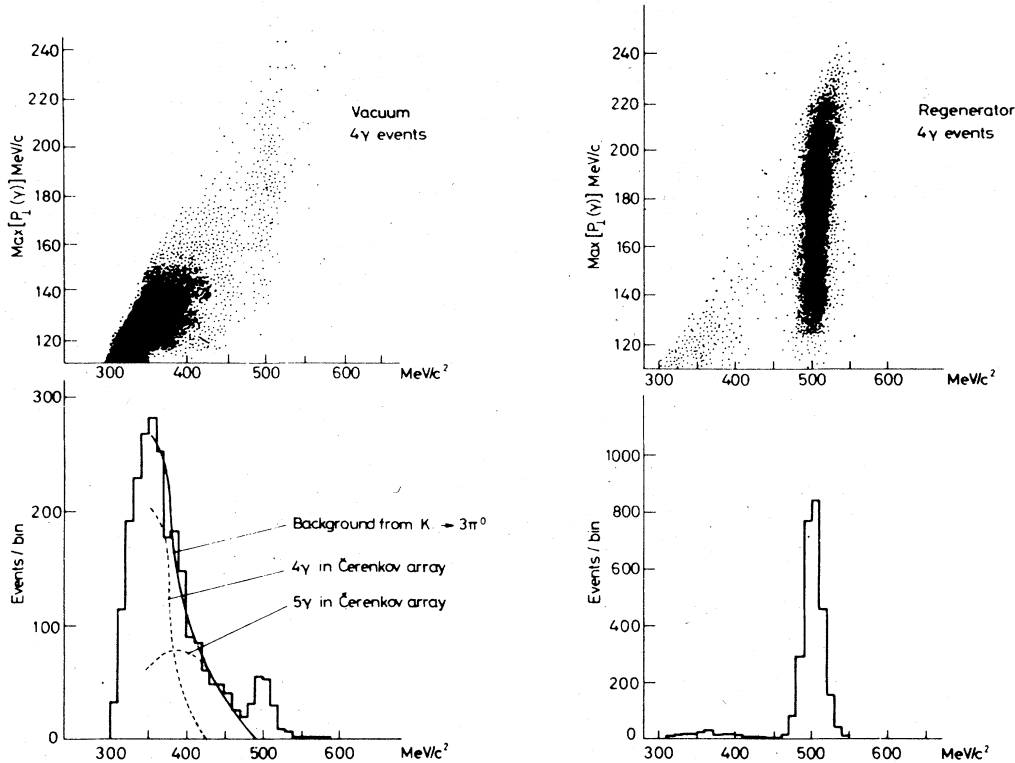
FIG. 4. Distributions of reconstructed K_L \rightarrow \pi^0 \pi^0 events, and regenerated K_S \rightarrow \pi^0 \pi^0 events.
