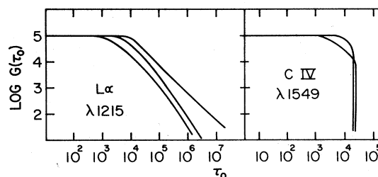
FIG. 8. Generating functions for the L\alpha and C IV \lambda 1549 resonance lines in thick photoionized regions, according to Ferland and Netzer (1979). These functions describe the production of resonance-line photons per unit optical depth \tau_0 at line center. Note that the C IV \lambda 1549 production region is distinctly limited in \tau_0 , but collisional excitation in the \text{H}^0 zone produces some L\alpha emission even for \tau_0 > 10^5 .
