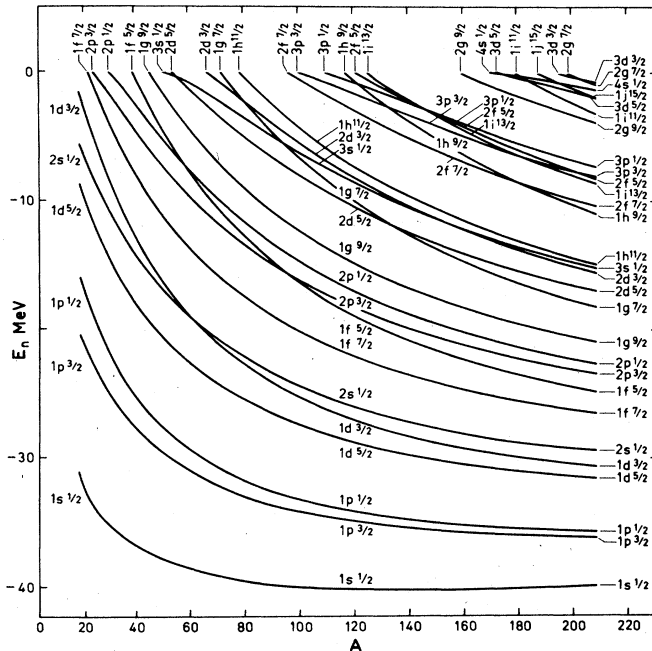
FIG. 2. Energies of neutron orbits using a model of C. J. Verje (from Bohr and Mottelson, 1969, Vol. I, p. 239, courtesy of W. A. Benjamin, Inc.). The least bound nucleons have energy \sim (-8 \text{ MeV}) which is small compared with their potential or kinetic energies inside the nucleus.
