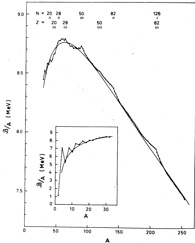
FIG. 1. The average binding energy per nucleon is plotted for nuclei stable against \beta decay. It is compared with the semi-empirical formula B/A = [15.56 - 17.23 A^{-1/3} - 23.28(N - Z)^2/A^2] \text{ MeV} - 3Z^2 e^2/5 R_0 A , with R_0 = 1.24 A^{1/3} \text{ fm} . This figure is from Bohr and Mottelson (1969 and 1975), courtesy of W. A. Benjamin, Inc.
