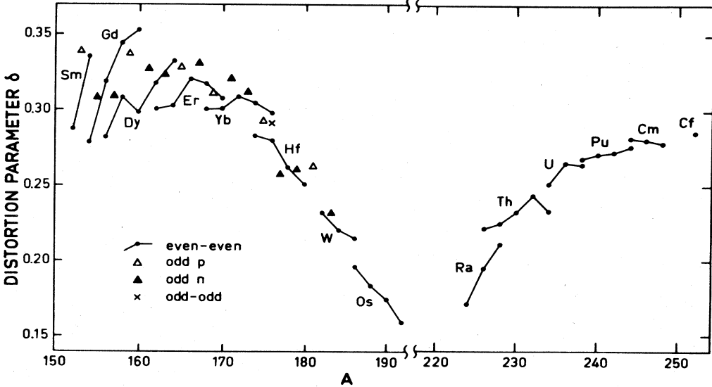
FIG. 5. A plot of the experimental distortion parameter \delta ( \approx \beta of this paper) in the rare earth region and beyond mass \sim 220 . [From Bohr and Mottelson (1975), Vol. II.]
