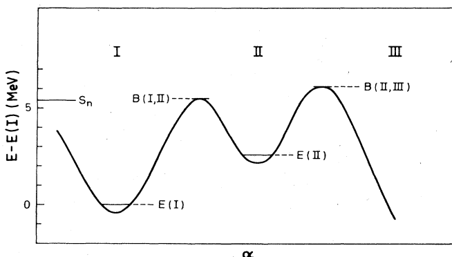
FIG. 8. Double hump energy vs distortion proposed by Strutinski to explain the observed features in subthreshold nuclear fission. [From Bohr and Mottelson (1975), Vol. II.]
