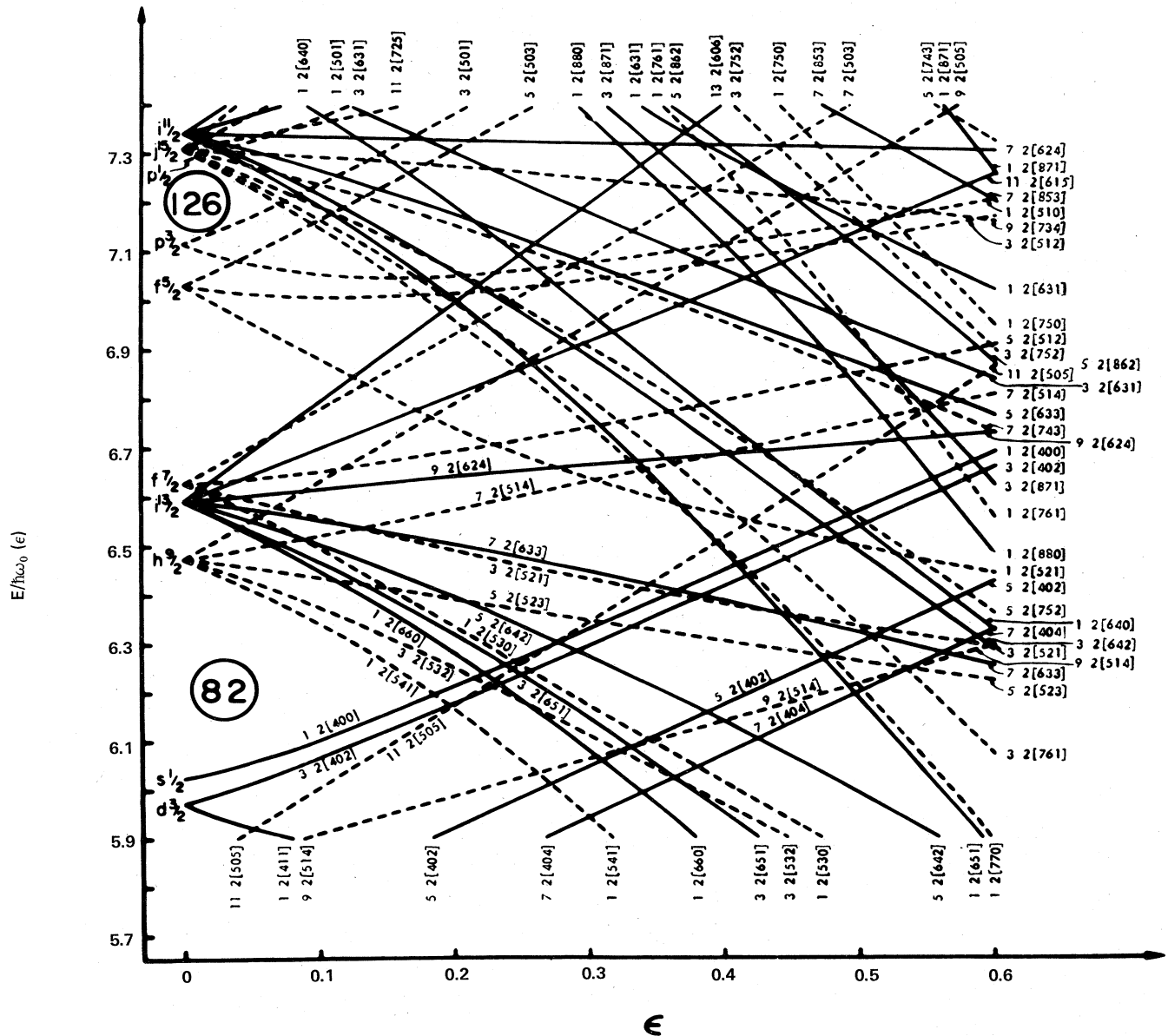
FIG. 6. Nilsson Diagram of single-particle shell-model proton states vs distortion for Z > 82 .
