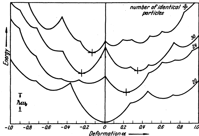
FIG. 7. Deformation potentials for various stages of shell filling-spheroidal harmonic oscillator binding potential. [S. A. Moszkowski (1957), Fig. 25.]
