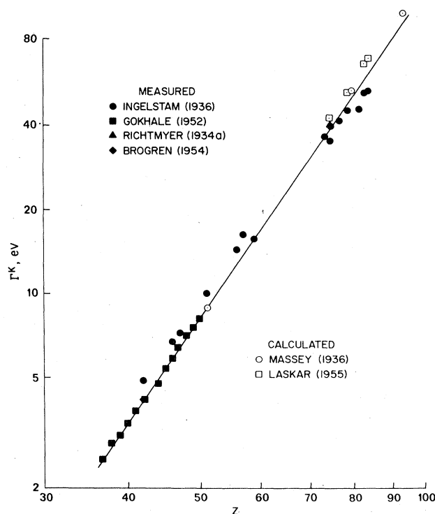
FIG. 2-11. K -level width as a function of atomic number. The straight line represents Eq. (2-65). [After Leisi, Brunner, Perdrisat, and Scherrer (1961), courtesy of Birkhauser Publishing Co.]
