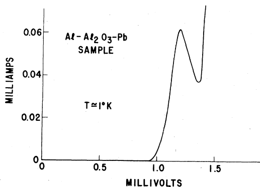
FIG. 11. A negative resistance characteristic obtained experimentally in tunneling between two different superconductors.
