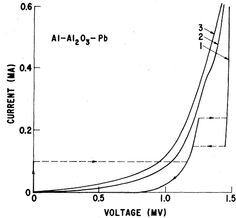
FIG. 13. Effect of trapped magnetic field on a tunneling characteristic. Curve 1 is a virgin curve, while Curve 3 is in a moderate magnetic field, and in Curve 2 the magnetic field has been removed. In Curve 1 we also have a small resistanceless current which we interpreted as caused by metallic shorts. In retrospect, it was actually due to the Josephson effect.
