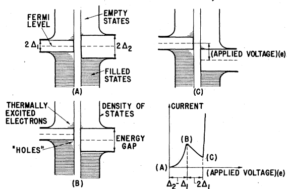
FIG. 10. Tunneling between two superconductors with different energy gaps at a temperature larger than 0^\circ \text{K} . (a) No voltage is applied between the two conductors. (b) As a voltage is applied it becomes energetically possible for more and more of the thermally excited electrons to flow from the superconductor with the smaller gap into the superconductor with the larger gap. At the voltage shown all the excited electrons can find empty states on the right. (c) As the voltage is further increased, no more electrons come into play, and since the number of states they can tunnel into decreases, the current will decrease as the voltage is increased. When the voltage is increased sufficiently the electrons below the gap in the superconductor on the left face empty states on the right, and a rapid increase in current will occur. (d) A schematic picture of the expected current-voltage characteristic.
