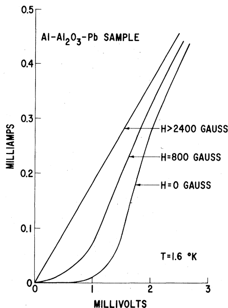
FIG. 8. The current-voltage characteristic at 1.6° K as a function of the applied magnetic field. At 2400 G the films are normal, at 0 G the lead film is superconducting. The reason for the change in the characteristics between 800 G and 0 G is that thin films have an energy gap that is a function of the magnetic field.
