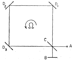
FIG. 1. Schematic of Sagnac's interferometer. A=light source; B=observer; C=beam splitter (half-silvered mirror); D 1 , D 2 , and D 3 are corner mirrors.
