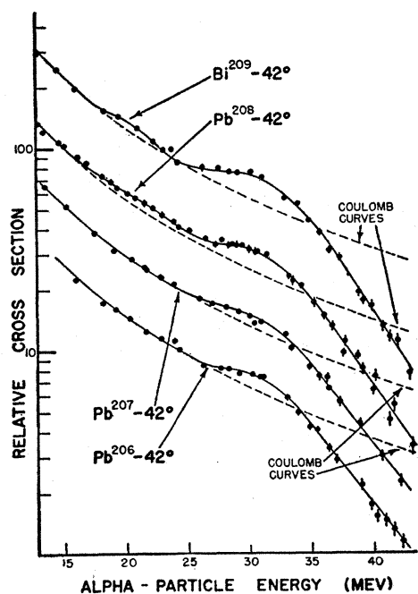
FIG. 3. Cross section 10 vs energy for elastic scattering of alpha particles from Pb 206 , Pb 207 , Pb 208 , and Bi 209 at 42° (in the laboratory system).
