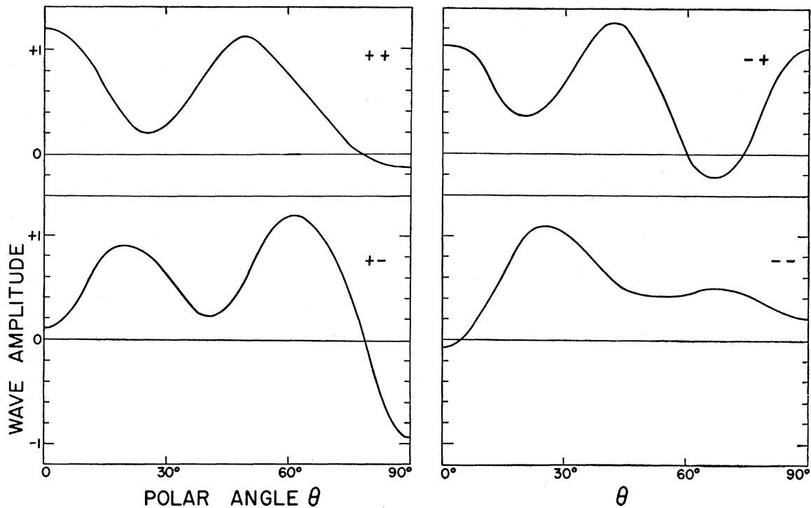
FIG. 6. Alpha wave functions are plotted vs polar angle on the spheroidal nuclear surface of \text{Cm}^{242} defined in the work of Rasmussen and Hansen. 22 Boundary conditions for the solutions at large distance are based on experimental relative intensities of alpha decay groups to 0, 2, 4, 6, and 8 spin states in the ground rotational band of the daughter. All cases represent a choice of l=0, 2, and 4 waves in phase (+) in the barrier, and the relative phases of l=6 and 8 waves are indicated by signs in the upper right-hand corner of each of the four plots.
