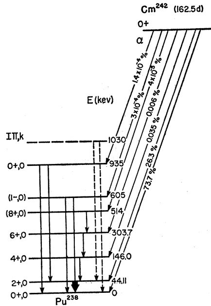
FIG. 7. Alpha decay scheme of \text{Cm}^{242} .
