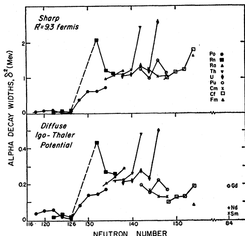
FIG. 5. Alpha decay reduced widths, \delta^2 , for ground-state transitions of all even-even alpha emitters are plotted against neutron number (of the parent nucleus). Barrier penetrabilities in the upper plot were calculated by the usual sharp cutoff of a pure coulombic potential, a cutoff radius of 9.3 \times 10^{-13} cm being chosen to give \delta^2 values in agreement with one-body theory. Barrier penetrabilities in the lower plot were calculated using a diffuse nuclear potential defined by the Igo-Thaler optical model parameters for 40-Mev alpha particles. 8
