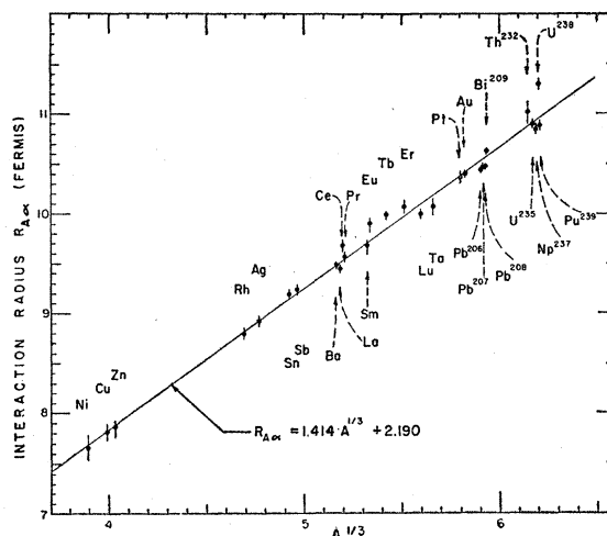
FIG. 4. Sharp cutoff radii from elastic scattering of alpha particles. 10 The radii are plotted against the cube root of the mass number. The straight line represents a least squares best fit.
