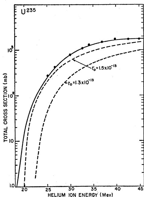
FIG. 1. Total reaction cross section 3 (fission plus spallation) vs energy for alpha-particle bombardment of U^{235} . The dashed curves are based on theoretical values of Blatt and Weisskopf 4 for two different choices of radius.
