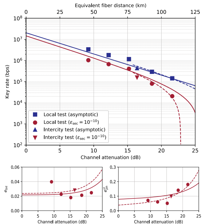
FIG. 3. Top: Experimental SKRs at different channel losses. The (blue) squares and upright triangles are asymptotic SKRs for the local test and the 43-km metropolitan intercity test, respectively. Similarly, the (red) circles and inverted triangles are the SKRs calculated within the composable security framework with \epsilon_{\text{sec}} = 10^{-10} for the local test and the metropolitan field test, respectively. In the local tests, a variable attenuator is used to provide higher attenuation beyond the channel's 0.2-dB loss. Solid and dashed lines correspond to numerical simulations of the SKRs for the local test and the intercity test, respectively. Bottom: Bit error rate ( e_{\text{bit}} ) and upper bound to the phase error rate ( e_{\text{ph}}^U ) against channel attenuation. The symbols used here are the same as the ones above.
