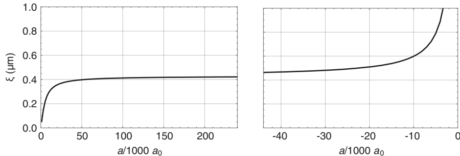
FIG. 12. Pair size \xi as a function of the scattering length. Linear densities \rho_0 from 1 to 3 atoms/ \mu\text{m} correspond to interparticle spacings from 1 to about 0.3 \mu\text{m} , which is of the order of the pair size. For higher densities and/or weaker interactions the pairs become larger than the interparticle separation and the mapping to a super-Tonks-Girardeau gas fails. Left and right panels correspond to positive and negative scattering lengths a .
