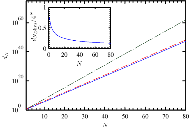
FIG. 11. Dimension of the physical subspace d_{N,\text{phys}} (blue solid line), the total number of basis states 4^N in our formulation (red dashed line), and the dimension of the basis from Ref. [55], 3^N(2j_{\text{max}} + 1)^{N-1} , for the simplest nontrivial truncation j_{\text{max}} = 1/2 (green dash-dotted line) as a function of system size. Inset: Fraction of the physical subspace with respect to the total amount of basis states.
