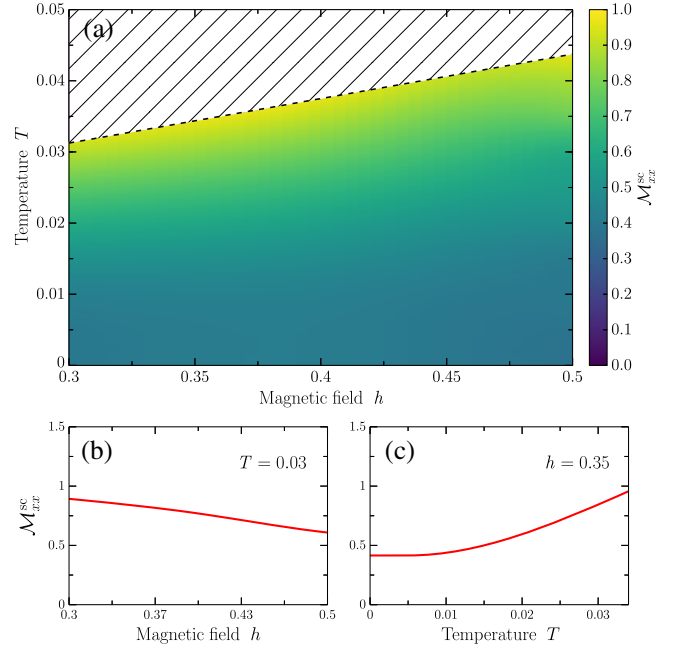
FIG. 9. (a) The colored surface represents the Skymion mass \mathcal{M}_{xx}^{sc} in the quantum regime calculated from Eq. (31) for \kappa = 0.1 , S = 1 , and \tilde{J}/\tilde{D} = 4 as a function of dimensionless magnetic field h and temperature T (for units, see text). The dashed line T = 2(\kappa + h/2)/(S(\tilde{J}/\tilde{D})^2) indicates the range of validity of Eq. (31). (b) Magnetic field dependence of \mathcal{M}_{xx}^{sc} for a fixed temperature T = 0.03 and (c) temperature dependence of \mathcal{M}_{xx}^{sc} for a fixed magnetic field h = 0.35 .
