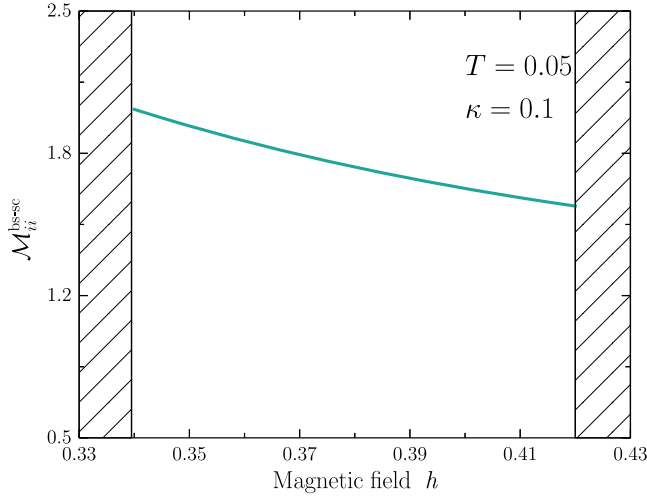
FIG. 8. Magnetic field dependence of diagonal mass tensor elements \mathcal{M}_{ij}^{bs-sc} for a Skymion with \kappa = 0.1 , at temperature T = 0.05 and for S = 1 and \tilde{J}/\tilde{D} = 4 . The magnetic field region where bound states contribute to the mass is bounded by the critical field below which the Skymion becomes unstable (left vertical line) up to the field where the bound state energy passes to the continuous spectrum (right vertical line).
