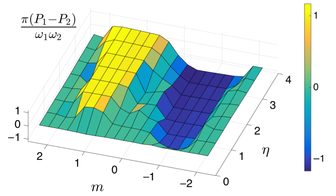
FIG. 5. Energy pumping between two frequency sources for varying \eta and m . The parameters of the system for this plot are \omega_1 = 0.1 and \omega_2 = \gamma\omega_1 . The pumping rate was averaged over the time range t < 10000 . The theoretical (ideal) value for the chosen parameters is |P_1 - P_2| = \omega_1 \omega_2 / \pi \approx 0.00515036 .
