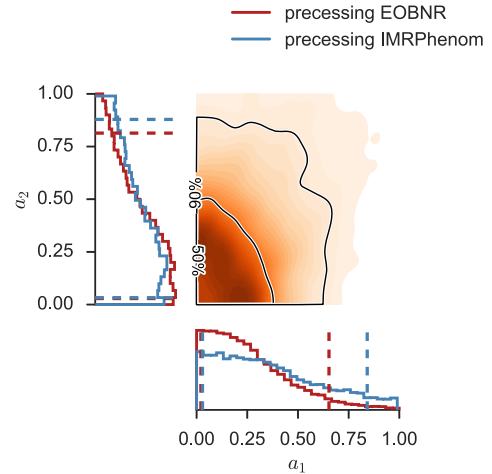
FIG. 3. Posterior probability densities for the dimensionless spin magnitudes. (See Fig. 2 for details.)
