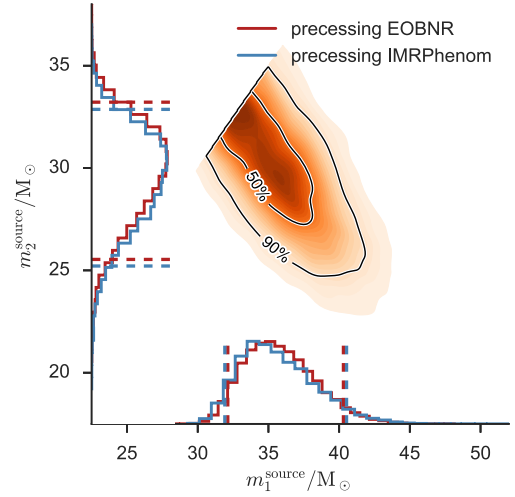
FIG. 2. Posterior probability densities for the source-frame component masses m_1^{\text{source}} and m_2^{\text{source}} , where m_2^{\text{source}} \leq m_1^{\text{source}} . We show one-dimensional histograms for precessing EOBNR (red) and precessing IMRPhenom (blue); the dashed vertical lines mark the 90% credible intervals. The two-dimensional density plot shows 50% and 90% credible regions plotted over a color-coded posterior density function.
