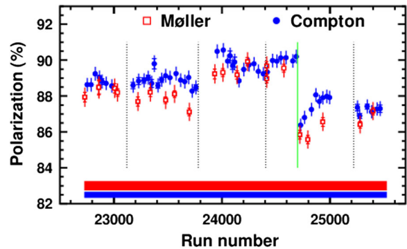
FIG. 7. The extracted beam polarization for the 1.16-GeV, 180- \mu\text{A} electron beam, as a function of run number and averaged over 30-hour-long periods, during the second-run period of the Q_{\text{weak}} experiment (blue, solid circle). Also shown are the results from the intermittent measurements with the Møller polarimeter [2] (red, open square). The inner error bars show the statistical uncertainty, while the outer error bar is the quadrature sum of the statistical and point-to-point systematic uncertainties. The solid bands show the additional normalization or scale-type systematic uncertainty (0.42% Compton and 0.65% Møller). The dashed and solid (green) vertical lines indicate changes at the electron source.
