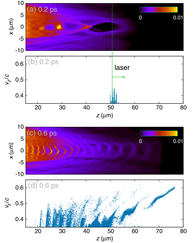
FIG. 4. Results of 3D PIC simulations with reconstructed laser wave front. Electron density n_e/n_c in the downward density ramp at the exit of the gas jet at (a) 0.2 and (c) 0.6 ps. (b), (d) Corresponding electron longitudinal phase space showing electron trapping and acceleration in the wakefield.
