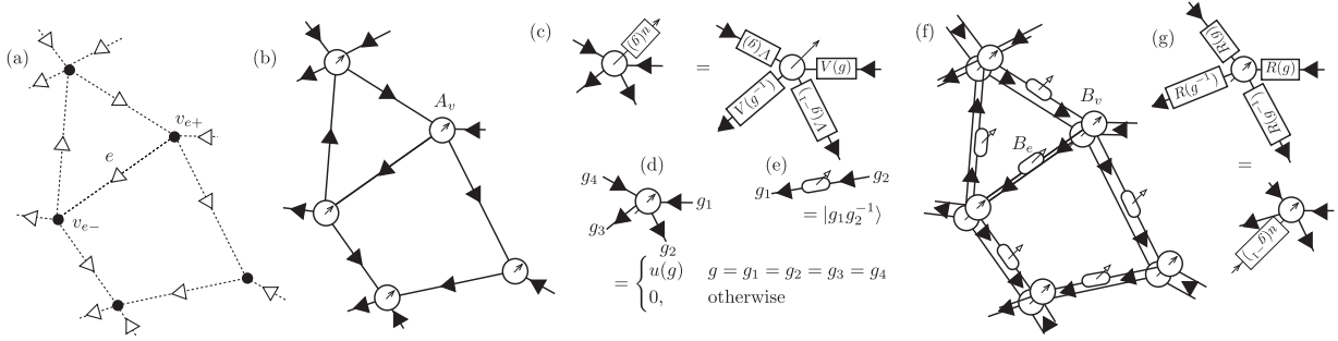
FIG. 1. (a) Definition of the graph \Lambda with vertices v and oriented edges e . (b) Construction of the PEPS |\psi(A)\rangle from tensors A_v associated with the vertices v and with virtual bonds along the edges e and physical indices depicted as arrows pointing out of the center of every tensor. (c) Symmetry of a PEPS tensor to ensure global symmetry of the state |\psi(A)\rangle under the group action U_g . (d) Definition of the tensor X_v used in the construction of the projector P onto the gauge-invariant subspace. (e) Result of acting with the tensor X_e on the physical input state |1\rangle , which is the only case we need throughout this manuscript. (f) PEPS |\Psi(B)\rangle with vertex tensors B_v and edge tensors B_e obtained from acting with P on |\psi(A)\rangle \otimes |1\rangle_e . (g) Symmetry property of the tensor X_v .
