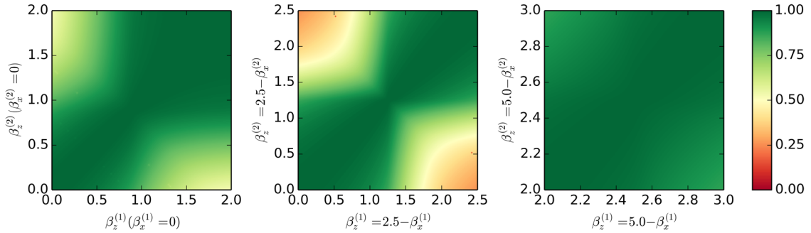
FIG. 3. Fidelity (per site) |\langle \Psi_{\boldsymbol{\beta}^{(1)}} | \Psi_{\boldsymbol{\beta}^{(2)}} \rangle|^{1/N} between any two ground states with parameters \boldsymbol{\beta} along the three different slices indicated in Fig. 2.
