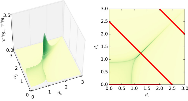
FIG. 2. Trace of the metric g(\boldsymbol{\beta}) with \boldsymbol{\beta} = (\beta_z, \beta_x) , as obtained from the fidelity |\langle \Psi_{\boldsymbol{\beta}} | \Psi_{\boldsymbol{\beta} + \delta\boldsymbol{\beta}} \rangle| = \exp(-N\delta\boldsymbol{\beta}^T g(\boldsymbol{\beta})\delta\boldsymbol{\beta}) , where N is the (infinite) number of sites, as defined in Ref. [80]. An analytic expression for g along the coordinate axes ( \beta_z = 0 or \beta_x = 0 ) was obtained in Ref. [81]. The red lines in the right panel indicate the slices studied in Figs. 3 and 4.
