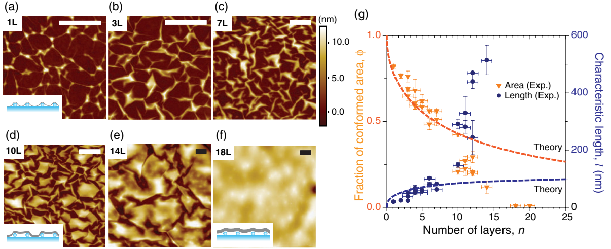
FIG. 6. Typical AFM images of (a) monolayer, (b) trilayer, (c) 7-layer, (d) 10-layer, (e) 14-layer, and (f) 18-layer graphene on \text{SiO}_2 with nanoparticle density 160 \pm 24 \mu\text{m}^{-2} . The scale bar in each image is 400 nm. The insets in (a), (d), and (f) are corresponding schematics of graphene films on nanoparticles to the AFM images. (g) The fractional area \phi where graphene conforms to the substrate and the characteristic length l of the delaminated domains, as functions of the number n of graphene layers. The dashed curves are the theoretical expectations for \phi (orange) and l (blue) (described in text).
