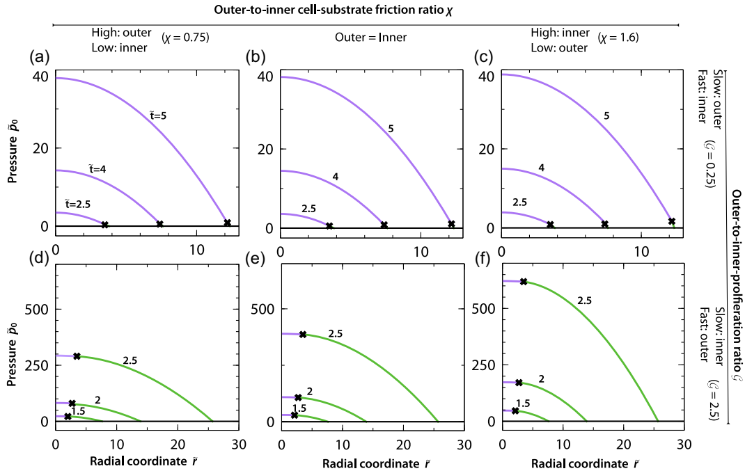
FIG. 9. Base 1D pressure field \tilde{p}_0 as a function of the radial coordinate \tilde{r} at different times for \mathcal{R} = 1.05 and different values of \mathcal{G} and \chi . Crosses indicate the position of the interface between the domains.
