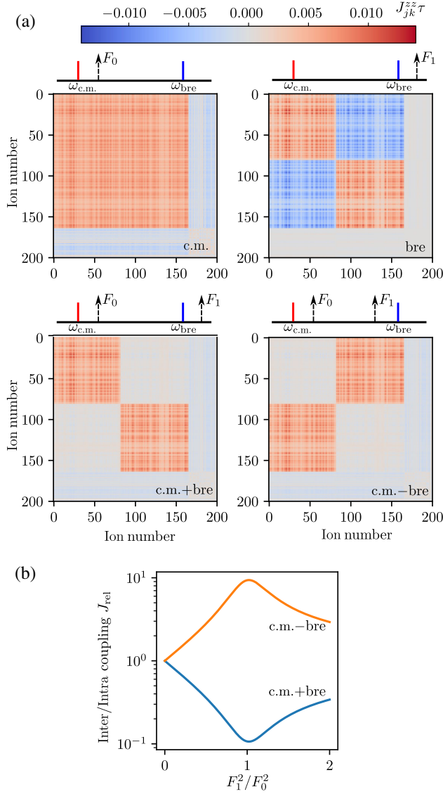
FIG. 10. On-the-fly control of intralayer and interlayer couplings using two-tone ODF. (a) Matrix of ion-ion couplings J_{jk}^z\tau generated by a single tone coupling only to the center-of-mass mode, a single tone coupling only to the breathing mode (“bre”), and two tones F_0 and F_1 of equal strength ( F_0 = F_1 ) respectively coupling to each mode with identical detunings (“c.m. + bre”) and with opposite detunings (“c.m. – bre”). The ion numbers are assigned based on whether an ion belongs to the top layer, the bottom layer, or the “scaffolding” structure, which respectively correspond to the ranges 0–81, 82–163, and 164–199. (b) Relative strength of interlayer-to-intralayer coupling, quantified by the metric J_{\text{rel}} [Eq. (31)], versus the relative weights of the two tones F_1^2/F_0^2 , for identical (c.m. + bre) and opposite (c.m. – bre) detunings. Here, we use the crystal shown in Fig. 4, ODF magnitude F_0 \approx 3.39 \times 10^{-23} N, detunings |\delta_0| = |\delta_1| \approx 2\pi \times 1.226 kHz, and \tau = 2\pi/|\delta_0| \approx 816 \mu\text{s} .
