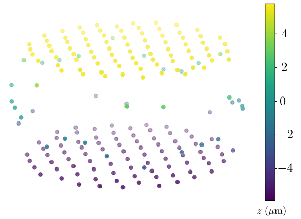
FIG. 1. Bilayer trapped-ion crystals for quantum information processing. We show a 3D view of a numerically obtained equilibrium configuration of a bilayer crystal with N = 200 trapped ions in a Penning trap. Markers, color coded according to the ion z coordinates, represent the ion positions. The trap center (not shown) is taken as the origin. In the lab frame, the crystal rotates with a controllable rotation frequency about a central axis that is normal to the layers, i.e., along the z direction. The crystal configuration is shown in the rotating frame. The trapping conditions under which this configuration is obtained are discussed in Sec. II B.
