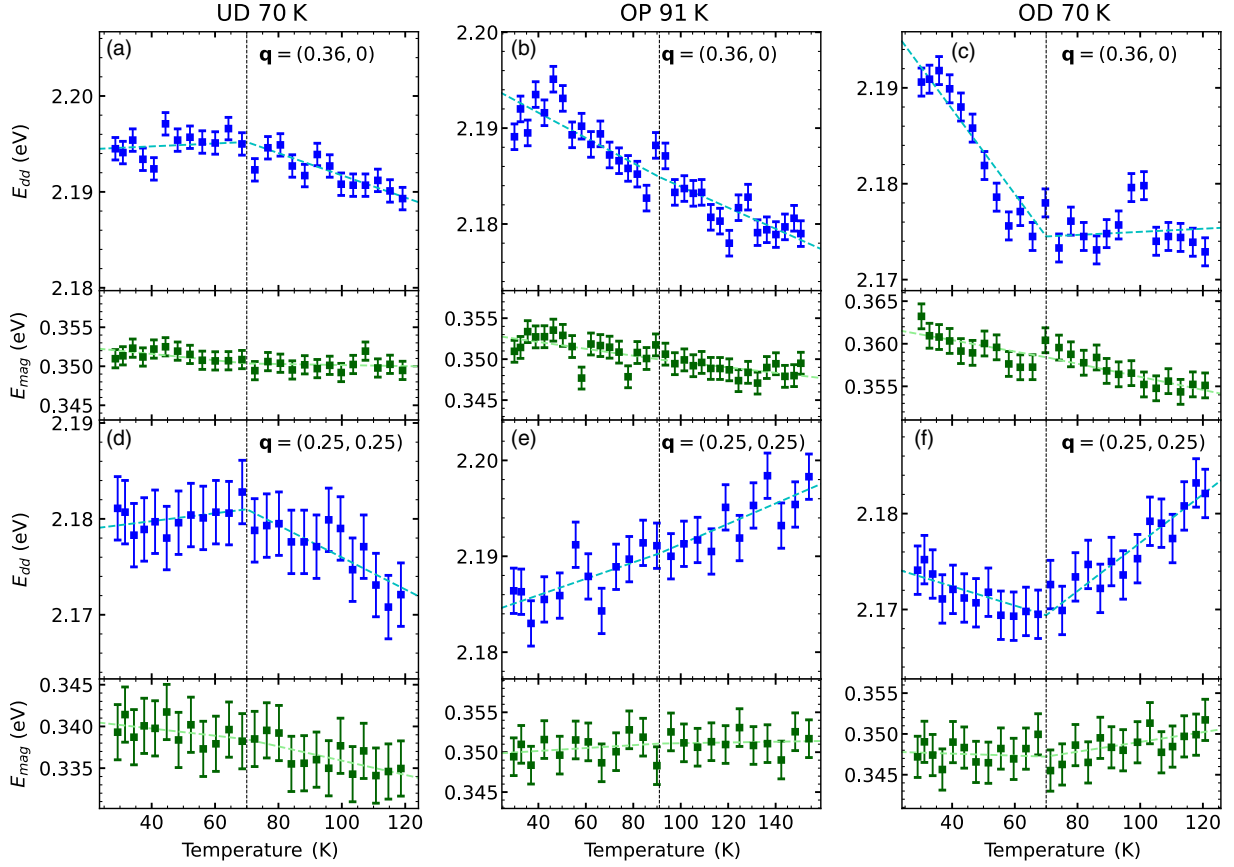
FIG. 3. Temperature dependence of the first moment of the dd exciton peak and the magnon peak, as extracted from the experimental spectra (considering, respectively, the energy intervals 1–4 and 0.1–0.6 eV). The dashed lines are fits to a curve parametrized as Eq. (2). The error bars represent the uncertainty on the elastic peak position computed as explained in Appendix A. The vertical dotted lines indicate T_c . Top panels: momentum value (0.36, 0). Bottom panels: momentum value (0.25, 0.25). (a),(d) Underdoped Bi-2212 ( T_c = 70 K). (b),(e) Optimally doped Bi-2212 ( T_c = 91 K). (c),(f) Overdoped Bi-2212 ( T_c = 70 K).
