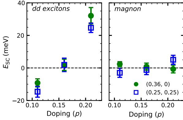
FIG. 5. Doping dependence of the superconductivity-induced change of the average \underline{d}d exciton and magnon energies. The momentum values are (0.36, 0) (green circles) and (0.25, 0.25) (blue squares). The error bars are extracted from the fit procedure.
