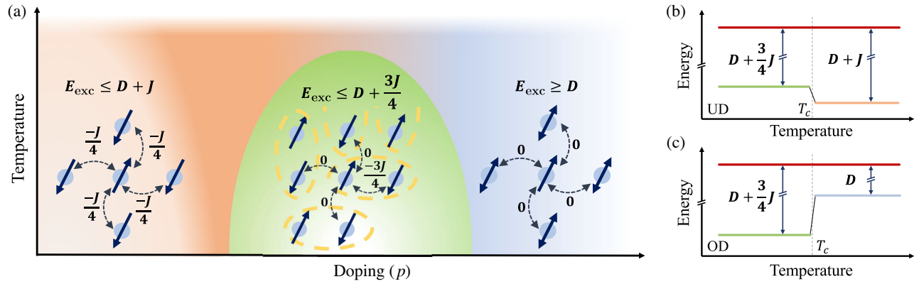
FIG. 6. (a) Phase diagram of the cuprates indicating the antiferromagnetic phase (beige), the normal phase (orange for underdoped and light blue for overdoped), and the superconducting phase (green) with the corresponding short-range spin correlations and \underline{d}\underline{d} exciton energies. (b),(c) Sketch of the temperature dependence of the \underline{d}\underline{d} exciton energy in the underdoped and overdoped cases.
