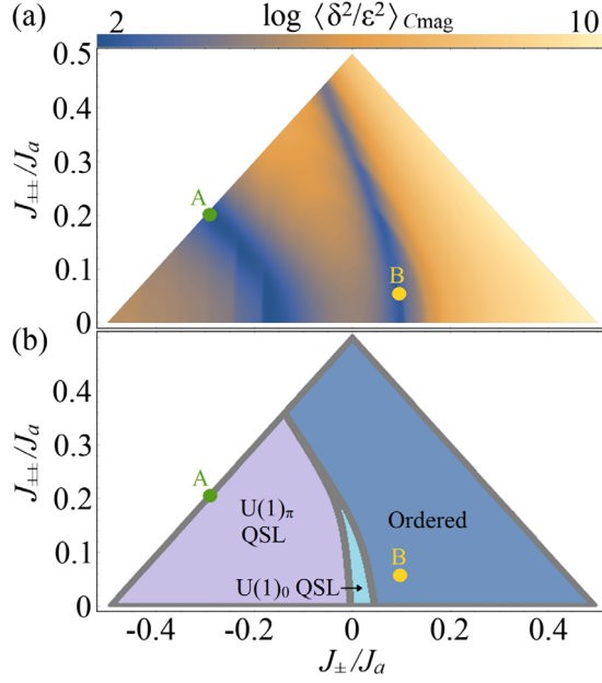
FIG. 4. (a) The goodness-of-fit parameter ( \langle \delta^2/\epsilon^2 \rangle_{C_{\text{mag}}} ) for the fourth-order NLC calculation compared to the measured C_{\text{mag}} , as a function of the exchange parameters, J_a , J_{\pm} = -\frac{1}{4}(J_b + J_c) , and J_{\pm\pm} = \frac{1}{4}(J_b - J_c) . This displays two local minima of \langle \delta^2/\epsilon^2 \rangle_{C_{\text{mag}}} . The best-fit parameters are labeled as parameter set A and parameter set B. The global minimum corresponds to set A while set B is only locally optimal. (b) The best-fit parameters from the NLC calculations (A and B) overlaid on the zero-field ground-state phase diagram predicted for the XYZ model Hamiltonian and DO pyrochlores [10]. The set A exchange parameters are well within the region of the phase diagram that is attributed to the U(1)_{\pi} QSL, while the set B parameters are well within the region attributed to an ordered ground state.
