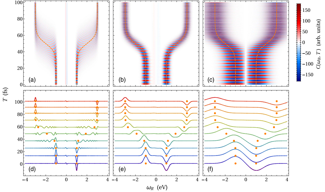
FIG. 9. STRUECARS signal for stochastic x-ray UDSP pulses with a < \pi . The correlation function in Eq. (37) is exhibited for \sigma = 10 eV and (a),(d) \tau = 19 fs, (b),(e) \tau = 4.7 fs, and (c),(f) \tau = 1.3 fs. The correlation function is shown (a)–(c) as a function of the time delay T and the Raman frequency \omega_R , and (d)–(f) for selected time delays. The orange dashed line in (a)–(c) and the orange dots in (d)–(f) display the time-dependent frequency \omega_{ba}(t) in Eq. (18). The mean frequency \omega_m must be such that |\omega_m| < \sigma . Here, we set \omega_m = 0 .
