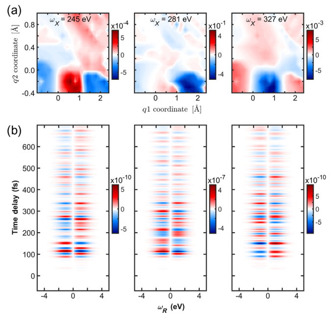
FIG. 13. Molecular polarizabilities of uracil and STRUECARS signal at three different probe wavelengths for z -polarized x -ray pulses. (a) Polarizability from Eq. (D7) in atomic units, in the two-dimensional nuclear space of the uracil Hamiltonian [59,60]. q_1 and q_2 are the nuclear degrees of freedom, with q_1 leading from the Franck-Condon point to the COIN, and q_2 leading to a local S_2 minimum. The indicated probe frequency enters Eq. (D7) as \omega_X , with the middle panel at 281 eV, 10 eV below the bound state carbon resonance, and the left and right panels significantly below and above this resonance, respectively. (b) STRUECARS signal associated with these polarizabilities. The same qualitative features are exhibited, with the signal in the middle panel being 3 orders of magnitude stronger than the other two.
