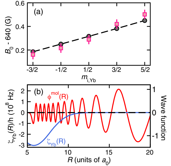
FIG. 4. (a) The observed (pink squares) and theoretically predicted (black circles) resonance locations near B = 640 G as functions of m_{i,\text{Yb}} . The ^6\text{Li} atom is in state |m_{s,\text{Li}}, m_{i,\text{Li}}\rangle = |-1/2, 0\rangle . For better visual comparison, the theoretical values have been uniformly shifted from those shown in Fig. 1(c). The shift is consistent with the 1.3 G uncertainty in the predicted resonance location. The dashed line is given by Eq. (7). (b) The ^{173}\text{Yb}^6\text{Li} hyperfine coupling coefficient \zeta_{\text{Yb}}(R) (solid blue line) and the radial wave function \phi^{\text{mol}}(R) of the most weakly bound state of the ^2\Sigma^+ potential (solid red line) as functions of separation R . Here, a_0 = 0.05292 nm is the Bohr radius.
