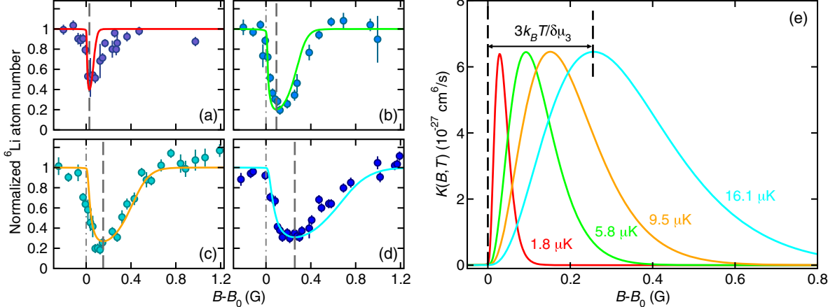
FIG. 5. Fermionic behavior of three-body recombination processes in {}^6\text{Li} and {}^{173}\text{Yb} mixtures found in atom-loss spectra and fitted theoretical line shapes as functions of magnetic field. {}^6\text{Li} is prepared in the |m_{s,\text{Li}}, m_{i,\text{Li}}\rangle = |-1/2, 0\rangle state and {}^{173}\text{Yb} in the |m_{i,\text{Yb}}\rangle = |+5/2\rangle state. The hold time is 4 s. Panels (a)–(d) correspond to the remaining {}^6\text{Li} atom number normalized to the remaining fitted {}^6\text{Li} atom number away from the resonance (markers with error bars) as a function of B - B_0 measured at temperatures of \{1.8, 5.8, 9.5, 16.1\} \mu\text{K} , respectively. The initial atom numbers for Li (Yb) are \{1.3(1.0), 1.7(3.3), 1.3, (2.0), 1.8(4.0)\} \times 10^5 and the initial peak densities for Li (Yb) are \{6.1(2.6), 12(8.3), 10(6.2), 11(9.3)\} \times 10^{12} \text{ cm}^{-3} . The fitted theoretical line shapes are the colored curves. We specify the magnetic field relative to the resonance location B_0 as determined from the fit. The dash-dotted and dashed lines, where given, locate the fitted resonance location B_0 and the field of maximum atom loss, respectively. The vertical axes are scaled to the theoretical background values away from the resonance. The magnetic moment of the trimer resonance state is \delta\mu_3 = 2.8\mu_B , while B_0 = 640.476 \text{ G} , A/k_B = 6 \times 10^{-6} \text{ nK} , and \Gamma_{\text{br}}/k_B = 100 \text{ nK} . The one-body loss rate is \Gamma_{\text{bg}} = 0.1 \text{ s}^{-1} for our lowest temperature and 0.075 \text{ s}^{-1} otherwise. Panel (e) shows the theoretical event rate coefficients as functions of B - B_0 for our four temperatures. The line colors correspond to those used in (a)–(d).
