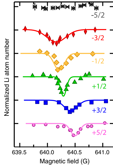
FIG. 3. Dependence of magnetic Feshbach resonances on the ^{173}\text{Yb} nuclear Zeeman state in a ^{173}\text{Yb}^6\text{Li} mixture seen in the remaining ^6\text{Li} atom number as functions of B near the 640 G Feshbach resonance. ^6\text{Li} is prepared in hyperfine state |m_{s,\text{Li}}, m_{i,\text{Li}}\rangle = |-1/2, 0\rangle and the ^{173}\text{Yb} sample is spin polarized in different nuclear Zeeman states. The data are normalized by the remaining ^6\text{Li} atom number away from resonance and vertically offset for clarity. The distance between vertical tick marks is one. From top to bottom ^{173}\text{Yb} is prepared in nuclear spin state m_{i,\text{Yb}} = -5/2, -3/2, -1/2, +1/2, +3/2 , and +5/2 . No resonance exists for m_{i,\text{Yb}} = -5/2 . The temperature is 1.8 \mu\text{K} ( 1.0 \mu\text{K} ) for Li (Yb) and the hold time is 1.5 s. Curves are best-fit Gaussians. Our full line shape analysis is found in Sec. VII.
